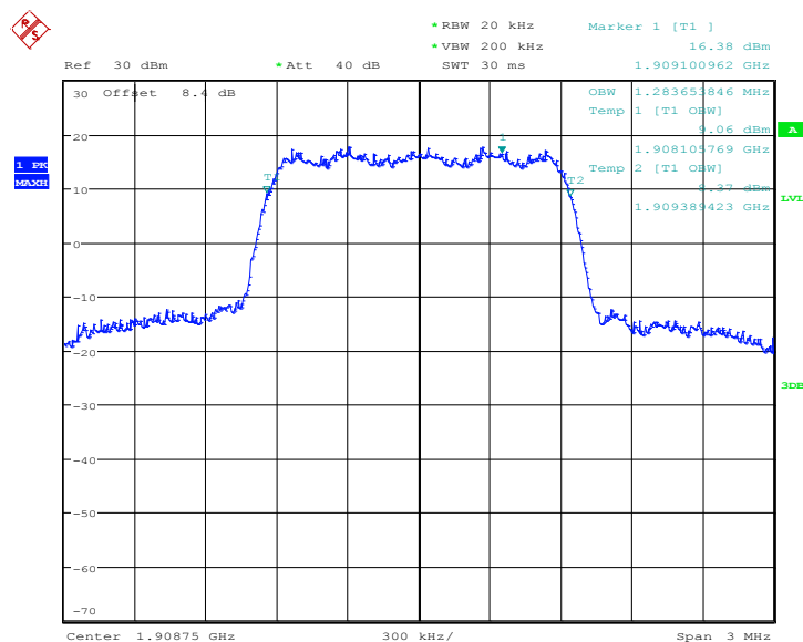
Fig.5 Channel 25-Occupied Bandwidth
