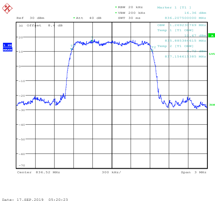
Fig.1 Channel 384-Occupied Bandwidth (99%)
