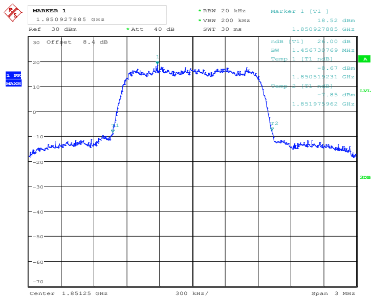
Fig.16 Channel 600- Emission Bandwidth (-26dBc BW)
