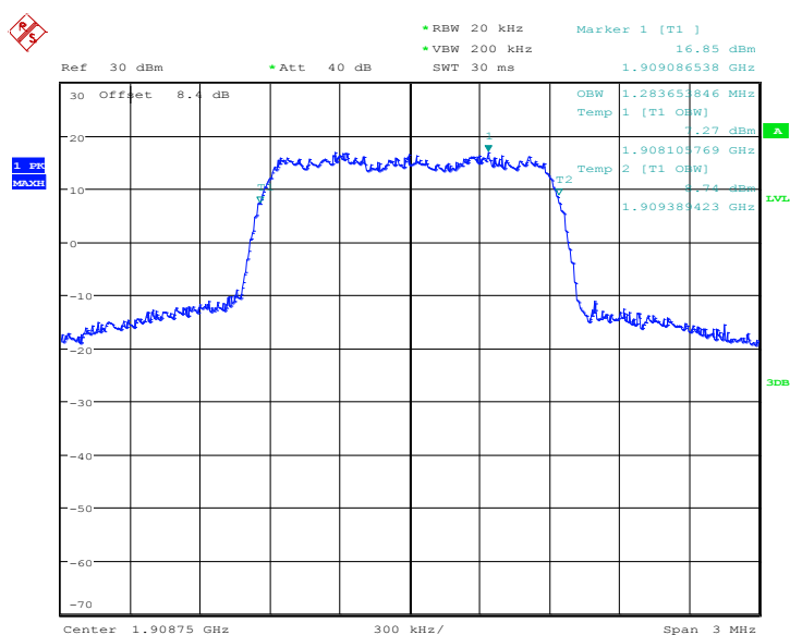
Fig.11 Channel 25-Occupied Bandwidth
