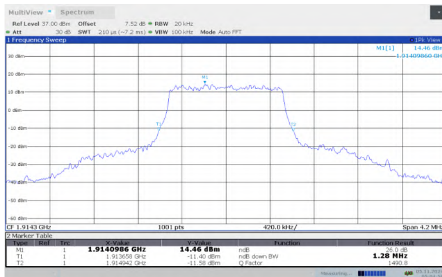
LTE band 25 , 1.4MHz Bandwidth, HIGH, 16QAM (-26dBc BW)
