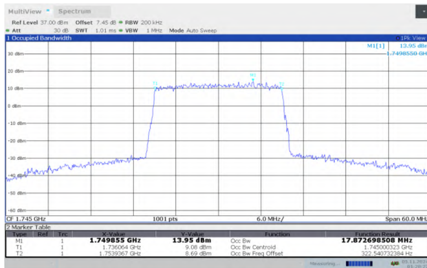
LTE band 4 , 20MHz Bandwidth, HIGH, 16QAM (99% BW)
