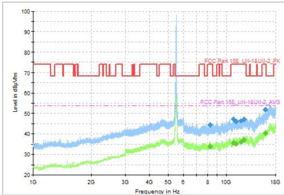
Fig. 56 Transmitter Spurious Emission (802.11ac-VHT40, CH102 5510MHz, 1GHz-18GHz)
