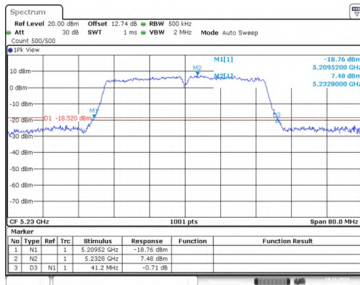
Fig. 4 Occupied 26dB Bandwidth (802.11ac-VHT40, 5230MHz)
