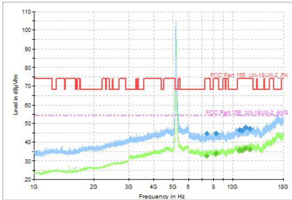
Fig. 52 Transmitter Spurious Emission (802.11ac-VHT40, CH38 5190MHz, 1GHz-18GHz)
