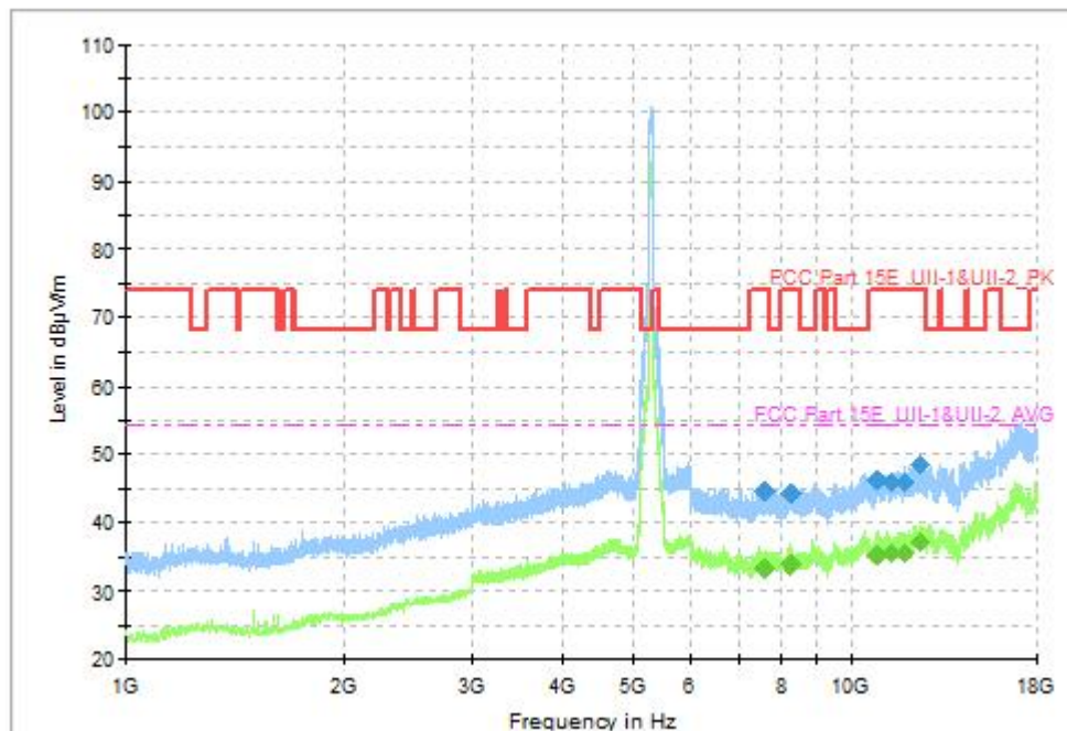
Fig. 62 Transmitter Spurious Emission (802.11ac-VHT80, CH58 5290MHz, 1GHz-18GHz)
