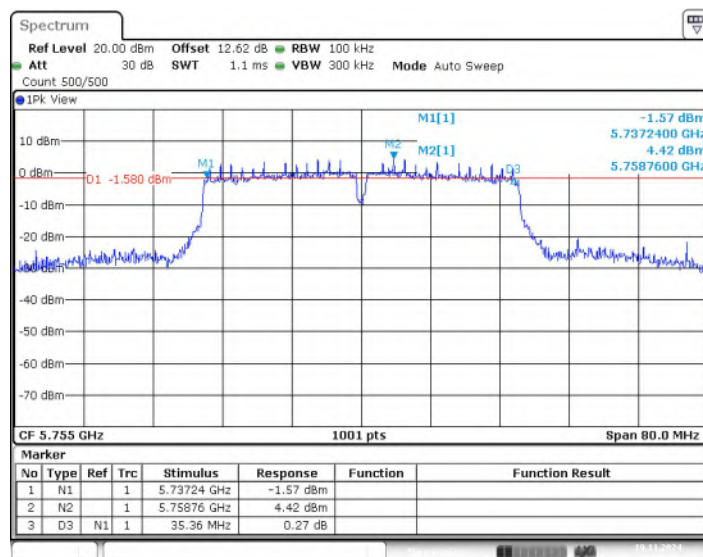
Fig. 10 Occupied 6dB Bandwidth (802.11ac-VHT40, 5755MHz)
