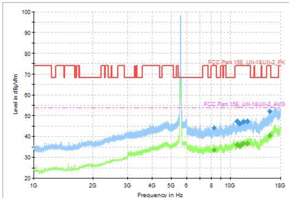
Fig. 57 Transmitter Spurious Emission (802.11ac-VHT40, CH118 5580MHz, 1GHz-18GHz)
