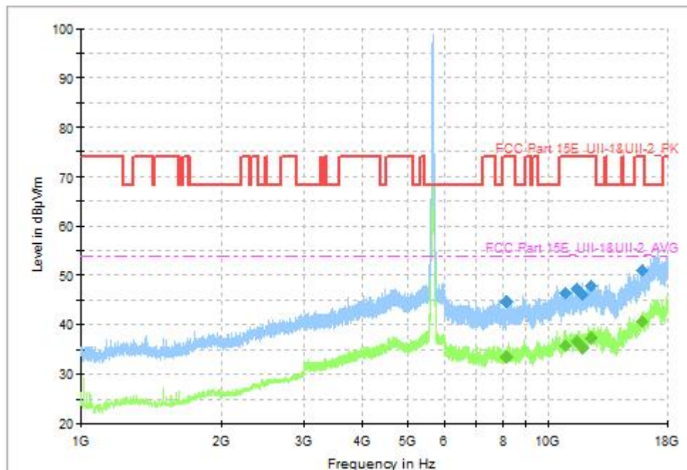
Fig. 58 Transmitter Spurious Emission (802.11ac-VHT40, CH134 5670MHz, 1GHz-18GHz)
