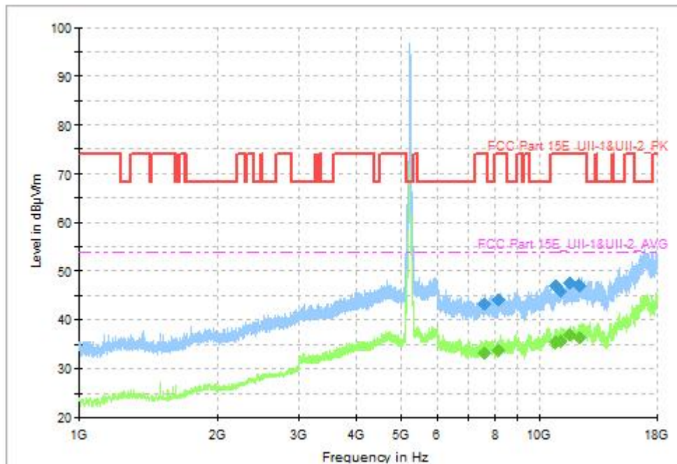
Fig. 53 Transmitter Spurious Emission (802.11ac-VHT40, CH46 5230MHz, 1GHz-18GHz)
