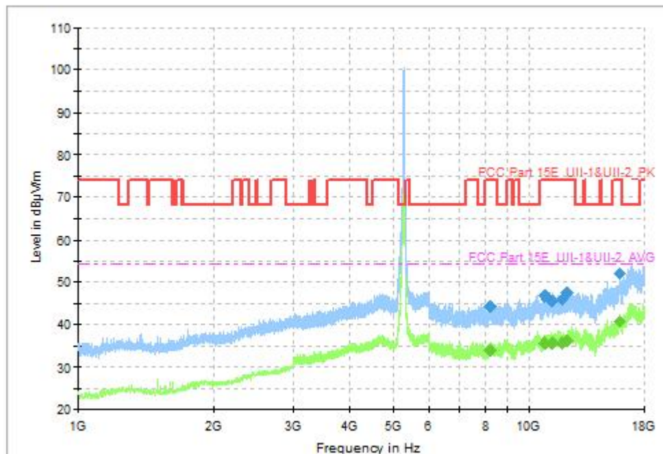
Fig. 54 Transmitter Spurious Emission (802.11ac-VHT40, CH54 5270MHz, 1GHz-18GHz)
