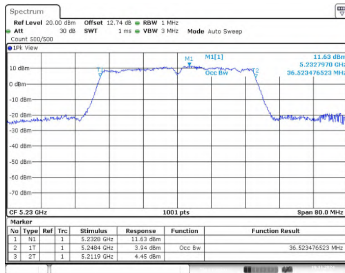
Fig. 16 99% Occupied Bandwidth (802.11ac-VHT40, 5230MHz)
