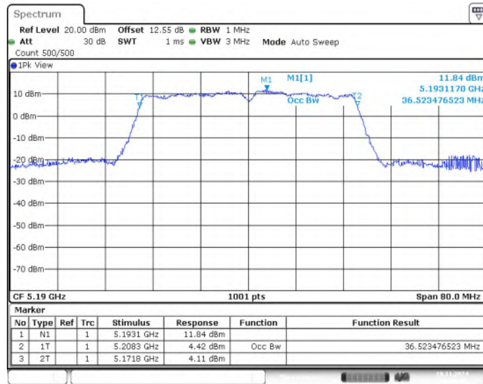
Fig. 15 99% Occupied Bandwidth (802.11ac-VHT40, 5190MHz)
