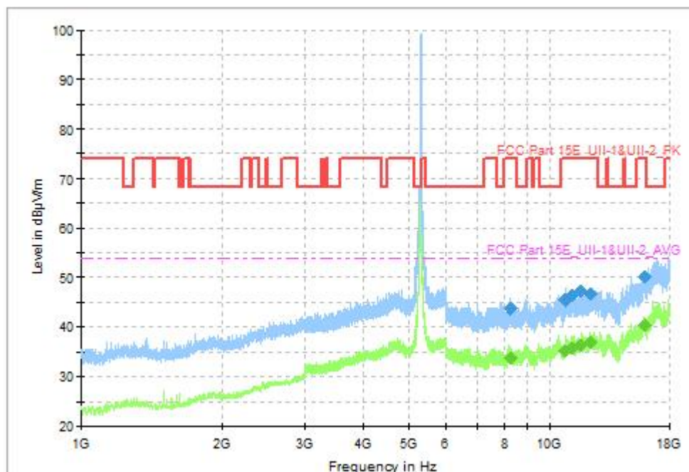
Fig. 55 Transmitter Spurious Emission (802.11ac-VHT40, CH62 5310MHz, 1GHz-18GHz)
