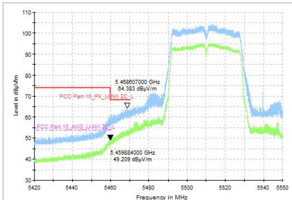
Fig. 31 Band Edges (802.11ac-VHT40, CH102 5510MHz)
