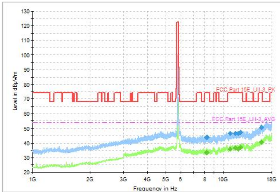
Fig. 60 Transmitter Spurious Emission (802.11ac-VHT40, CH159 5795MHz, 1GHz-18GHz)
