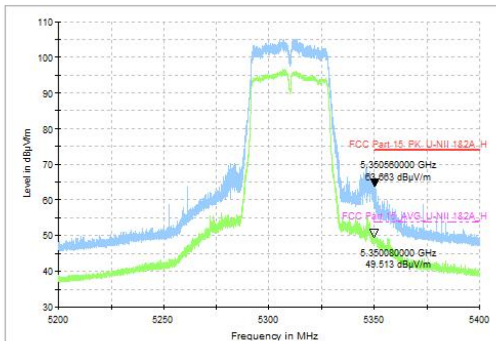
Fig. 30 Band Edges (802.11ac-VHT40, CH62 5310MHz)
