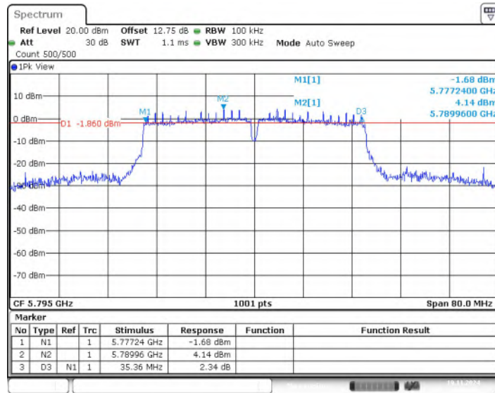
Fig. 11 Occupied 6dB Bandwidth (802.11ac-VHT40, 5795MHz)
