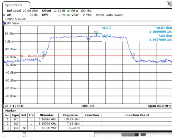
Fig. 3 Occupied 26dB Bandwidth (802.11ac-VHT40, 5190MHz)
