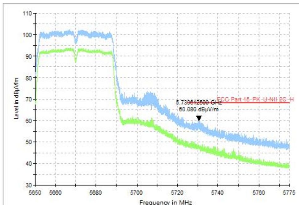
Fig. 32 Band Edges (802.11ac-VHT40, CH134 5670MHz)
