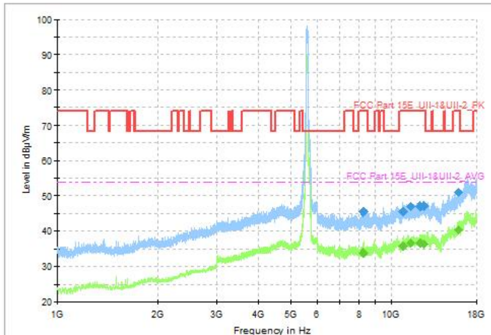
Fig. 64 Transmitter Spurious Emission (802.11ac-VHT80, CH122 5610MHz, 1GHz-18GHz)
