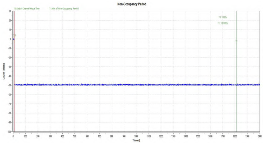
Fig. 21 Non-Occupancy Period (802.11a Frequency Band: 5250MHz ~ 5350MHz)
