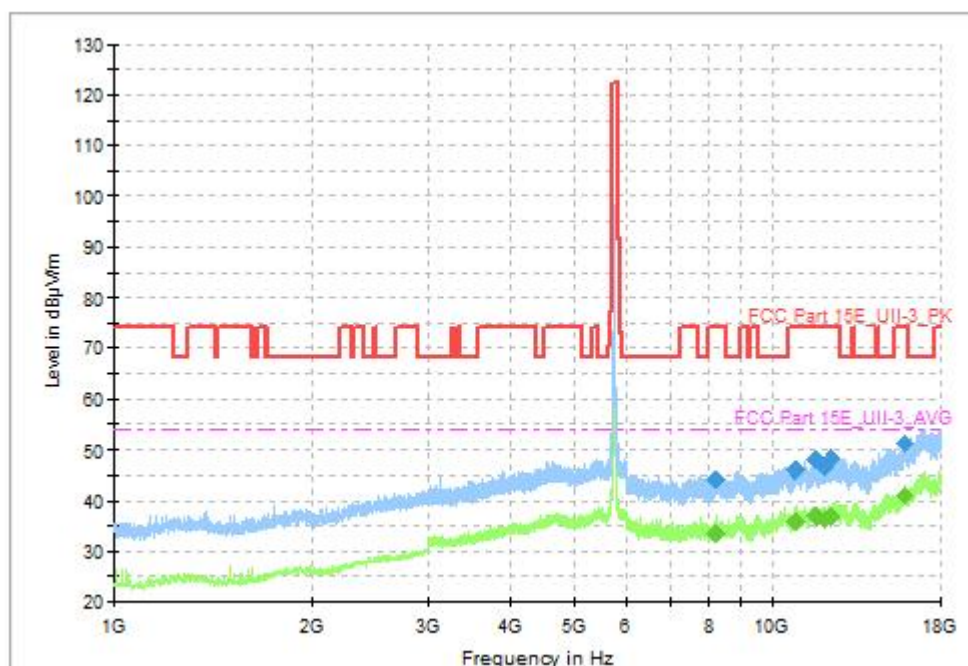
Fig. 59 Transmitter Spurious Emission (802.11ac-VHT40, CH151 5755MHz, 1GHz-18GHz)
