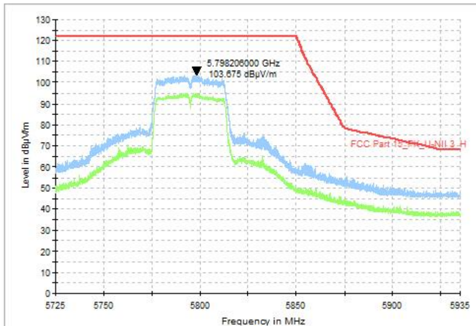
Fig. 34 Band Edges (802.11ac-VHT40, CH159 5795MHz)
