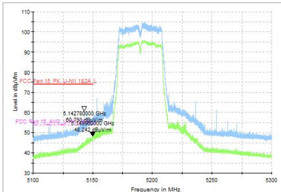
Fig. 29 Band Edges (802.11ac-VHT40, CH38 5190MHz)
