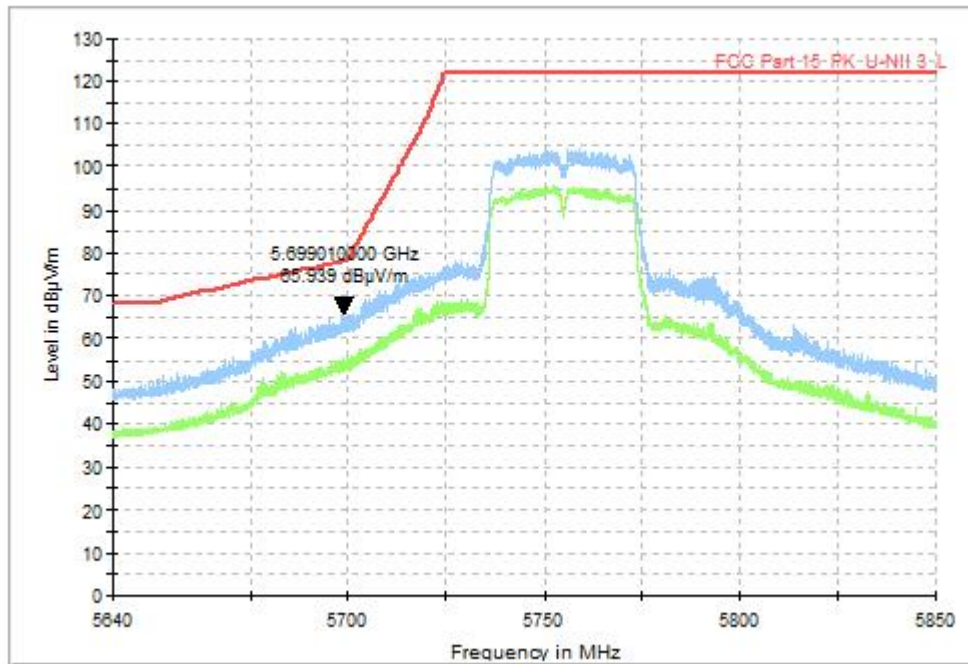
Fig. 33 Band Edges (802.11ac-VHT40, CH151 5755MHz)
