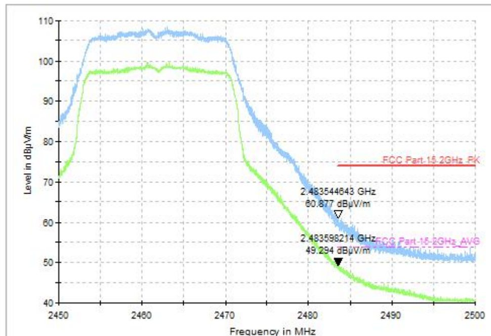
Fig.41 Radiated Restricted Band (802.11n-HT20, CH11, 2.45GHz~2.50GHz)
