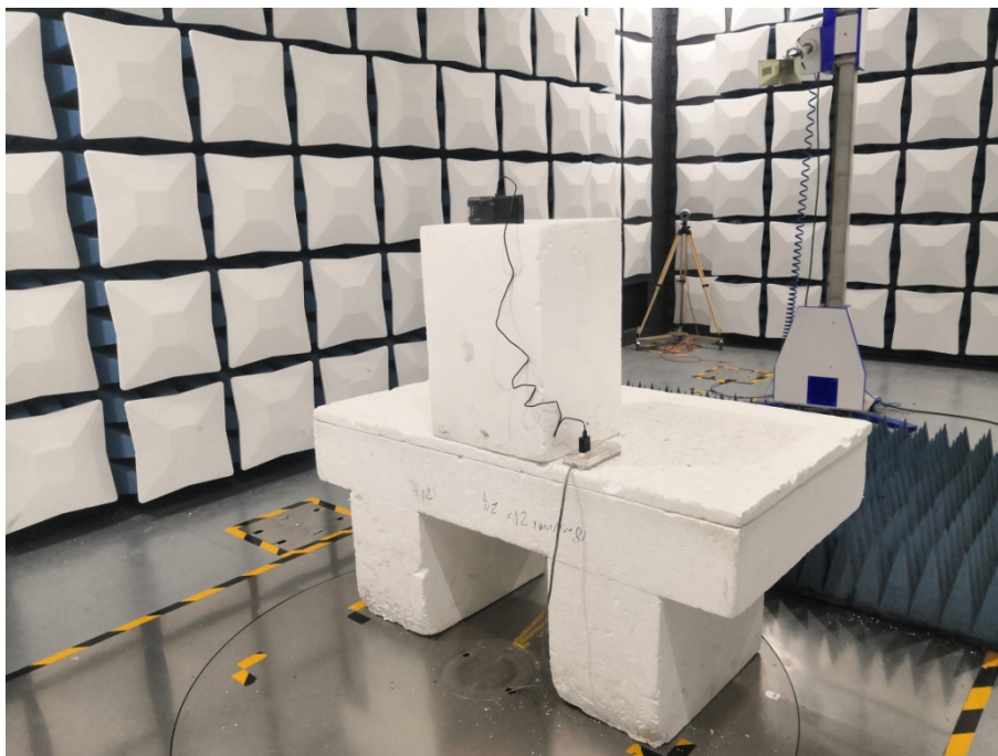
Radiated Emissions View (1-18G)
