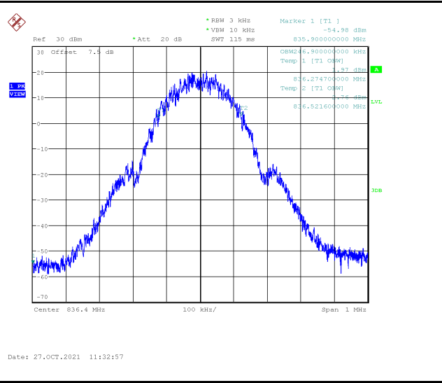
Channel 189-Occupied Bandwidth (99%)
