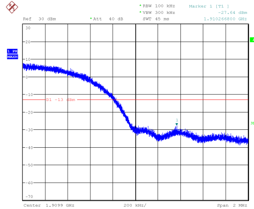
Channel 9538- HIGH BAND EDGE BLOCK
