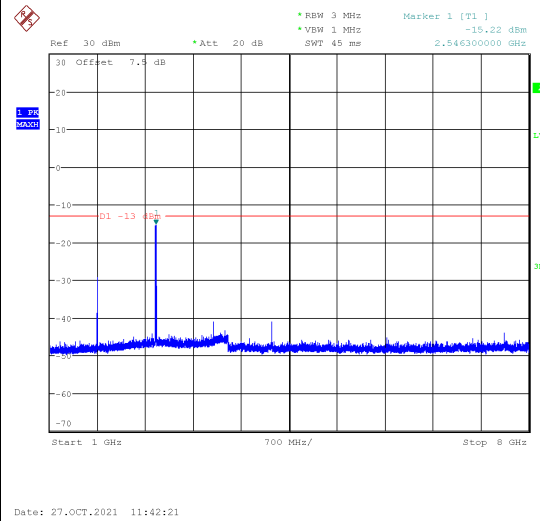
Channel 251: 1GHz~8GHz
