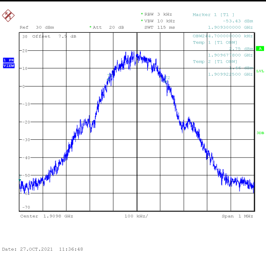
Channel 810-Occupied Bandwidth (99%)
