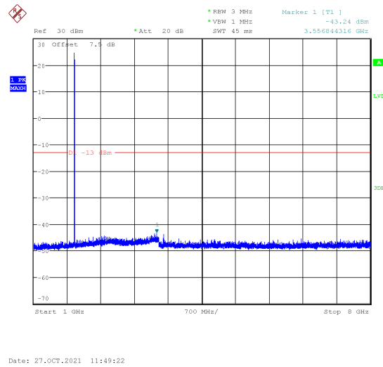
Channel 661: 1GHz~8GHz
