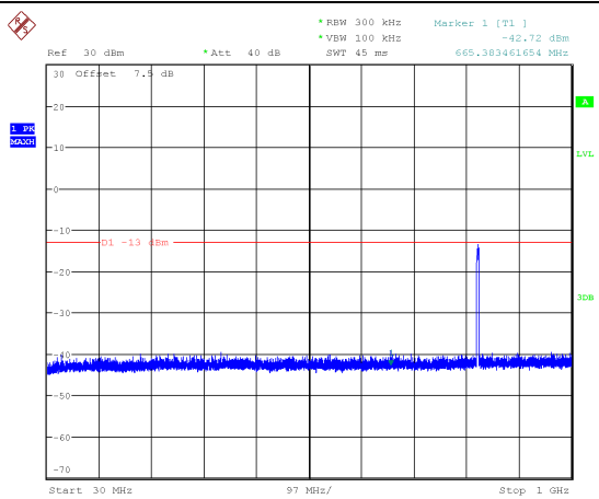
Channel 4232: 30MHz~1GHz
