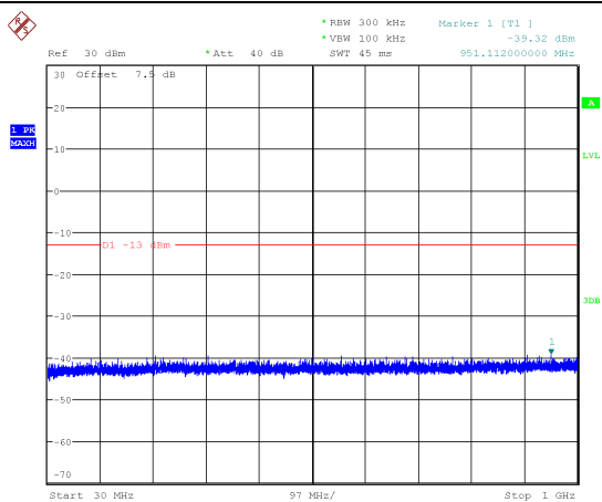
Channel 1512: 30MHz~1GHz
