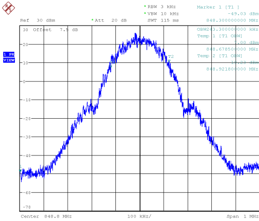
Channel 251-Occupied Bandwidth (99%)
