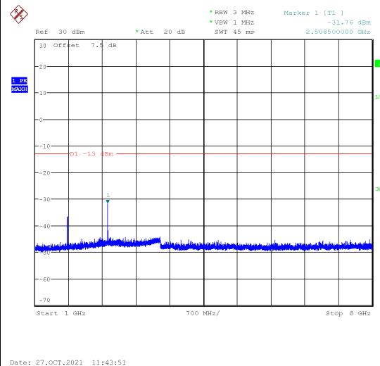
Channel 189: 1GHz~8GHz
