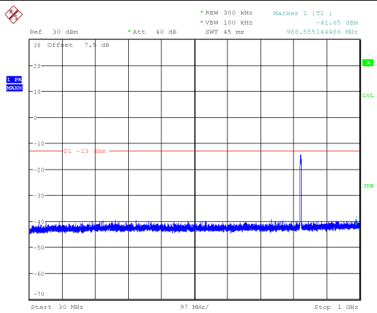
Channel 4175: 30MHz~1GHz
