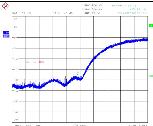
Channel 4132- LOW BAND EDGE BLOCK
