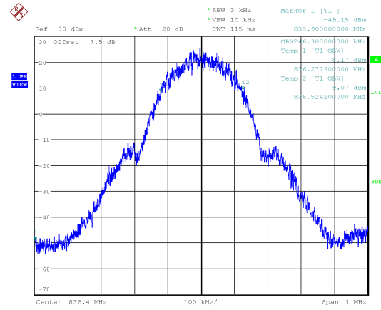
Channel 189-Occupied Bandwidth (99%)
