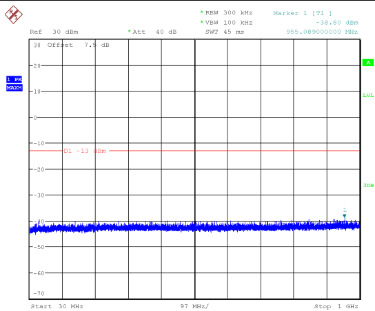
Channel 9400: 30MHz~1GHz
