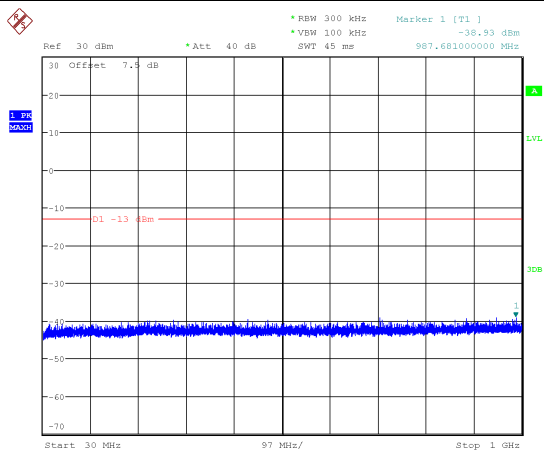
Channel 1450: 30MHz~1GHz
