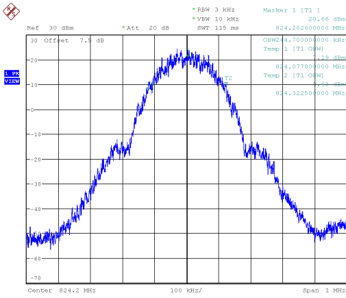
Channel 128-Occupied Bandwidth (99%)
