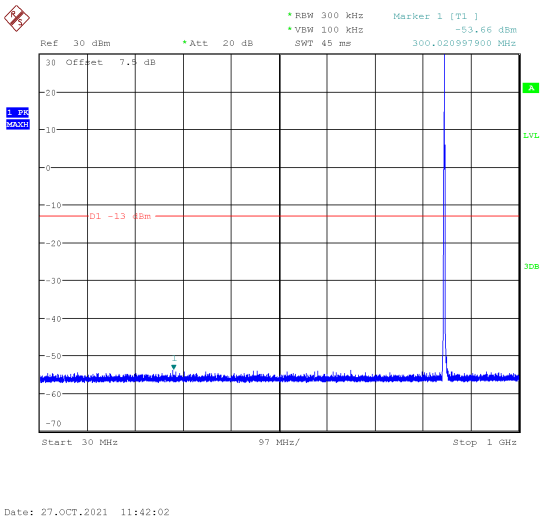
Channel 251: 30MHz~1GHz
