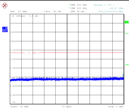
Channel 9537: 30MHz~1GHz
