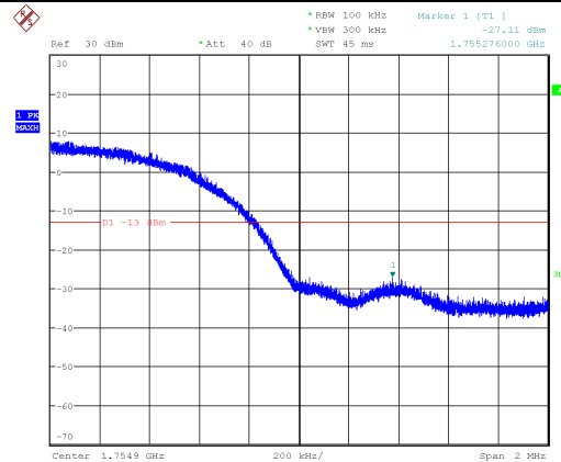
Channel 1513- HIGH BAND EDGE BLOCK
