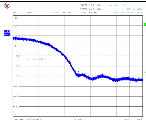
Channel 4233- HIGH BAND EDGE BLOCK
