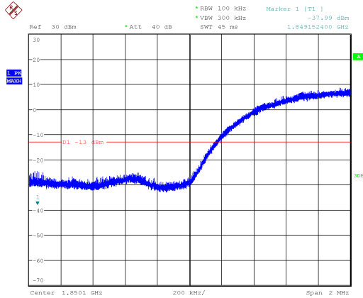
Channel 9262- LOW BAND EDGE BLOCK
