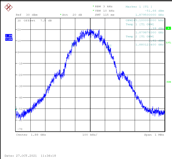
Channel 661-Occupied Bandwidth (99%)
