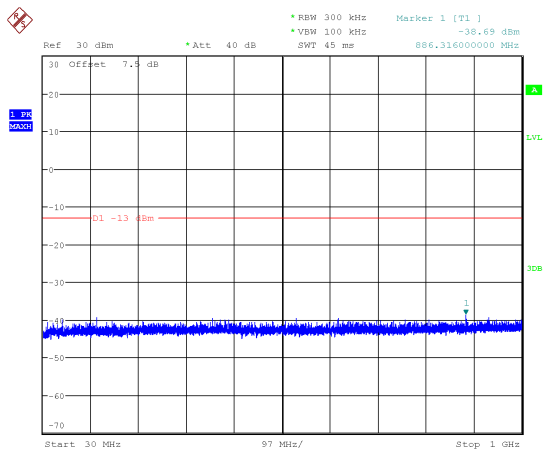
Channel 1313: 30MHz~1GHz
