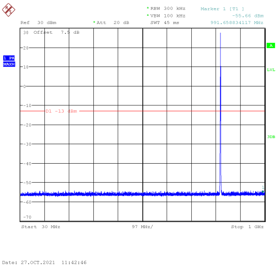
Channel 189: 30MHz~1GHz
