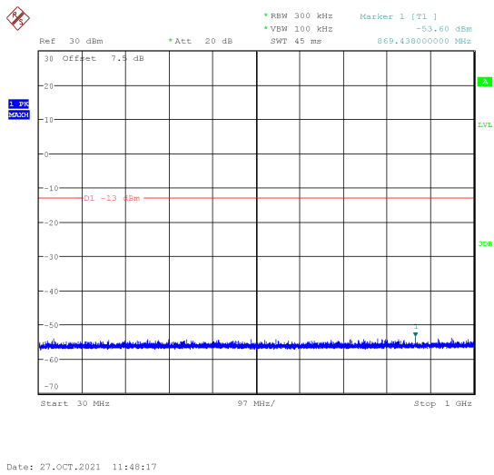
Channel 810: 30MHz~1GHz
