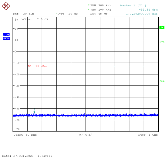
Channel 661: 30MHz~1GHz
