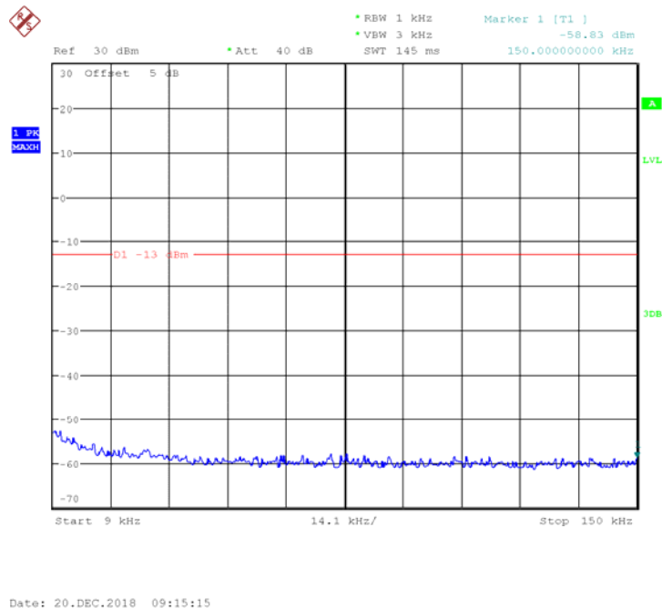
Fig.49 Channel 384: 9KHz~150KHz
