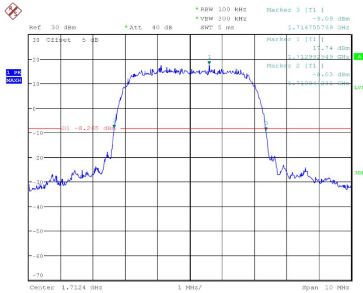
Fig.37 Channel 1413- Emission Bandwidth (-26dBc BW)
