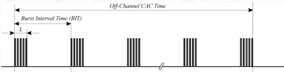
Pic 6-5: General structure of a multiple burst/packet based staggered PRF based radar test signal
