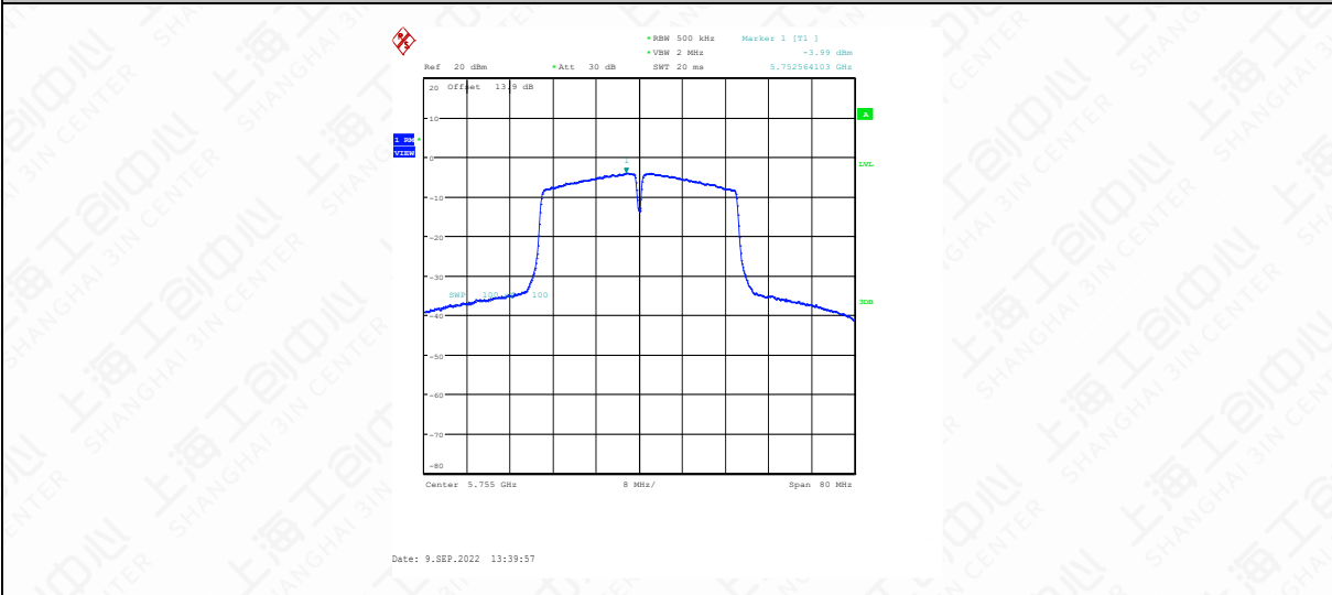
11AC40SISO-Ant1-5755--4.25-0.26-0.00-0.00
