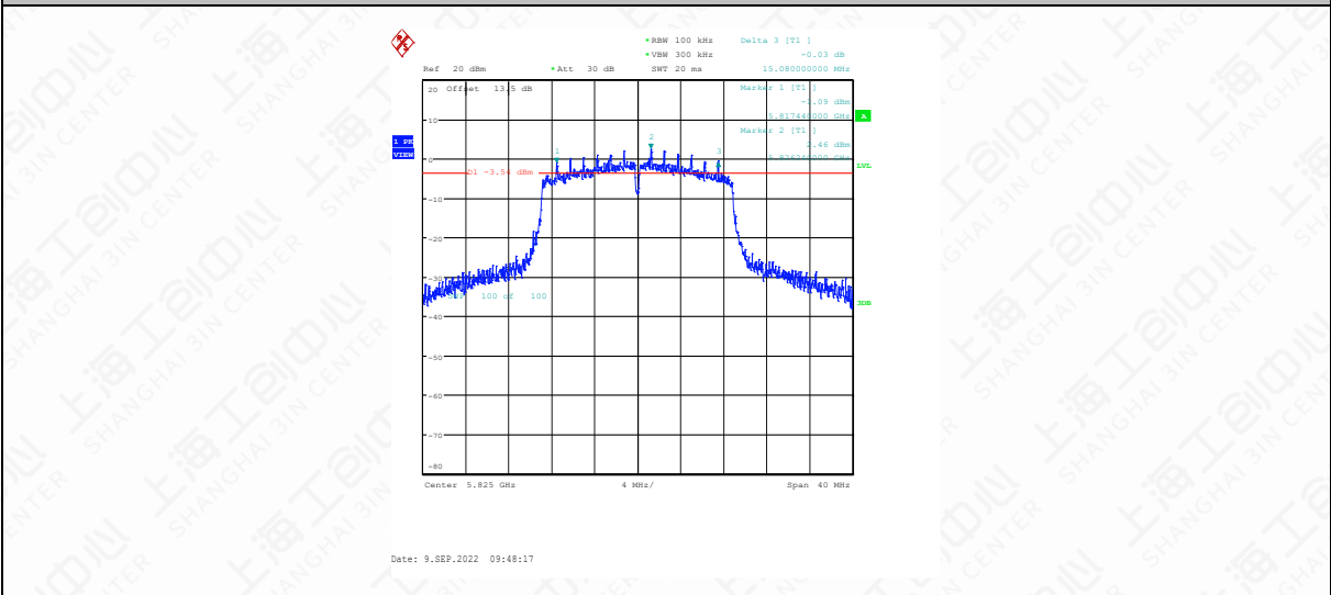
11N20SISO-Ant1-5825
