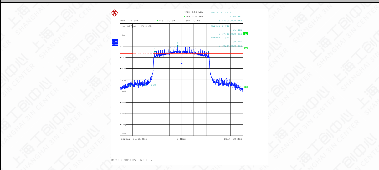
11N40SISO-Ant1-5795
