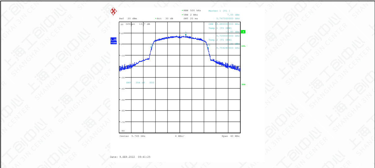
11N20SISO-Ant1-5745
