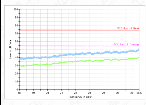
Radiated Spurious Emission (802.11b, Ch11, 18GHz~26.5GHz)
