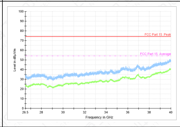
Radiated Spurious Emission (802.11b, Ch1, 26.5GHz~40GHz)
