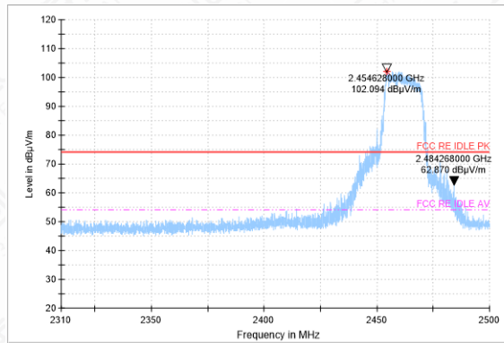
Peak detector
