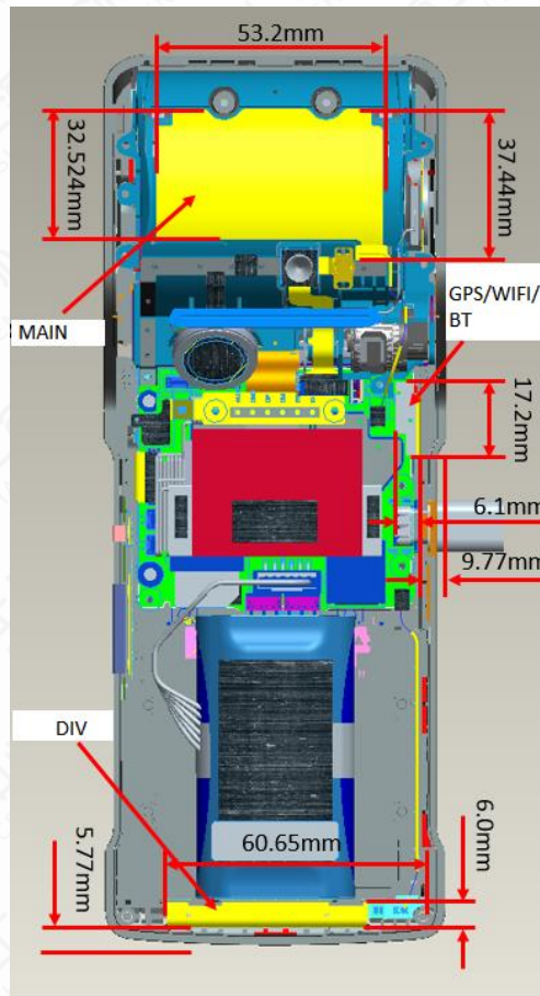
Figure 12.2-1 Antenna Locations
