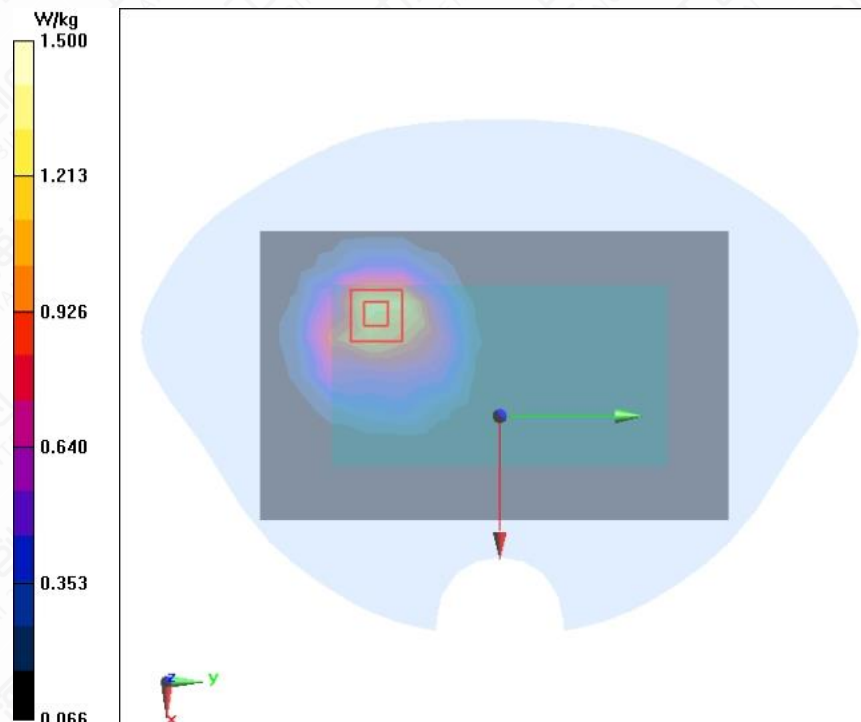
Figure A.2-1 GSM 850 GPRS 4TS Back Mode High 5mm
