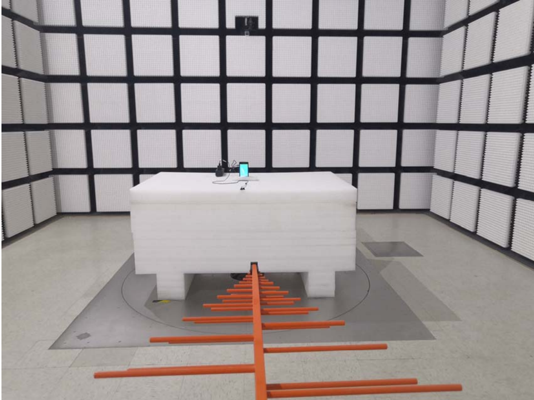
Radiated Emission Above 1GHz View Type-1 Adapter 1#
