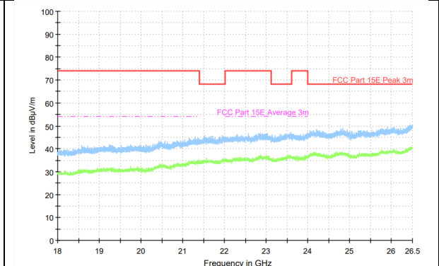
Radiated Spurious Emission (802.11n 20M-MIMO, ch52, 18GHz-26.5GHz)
