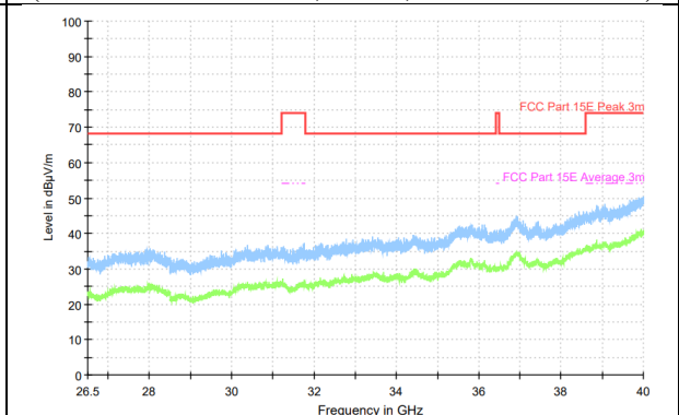
Radiated Spurious Emission (802.11ac 20M-MIMO, ch100, 26.5 GHz-40 GHz)
