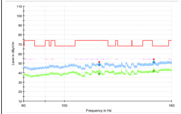
Radiated Spurious Emission (802.11ac 20M-MIMO, ch52, 8GHz-18GHz)
