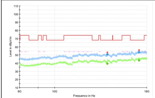
Radiated Spurious Emission (802.11n 20M-MIMO, ch52, 8GHz-18GHz)
