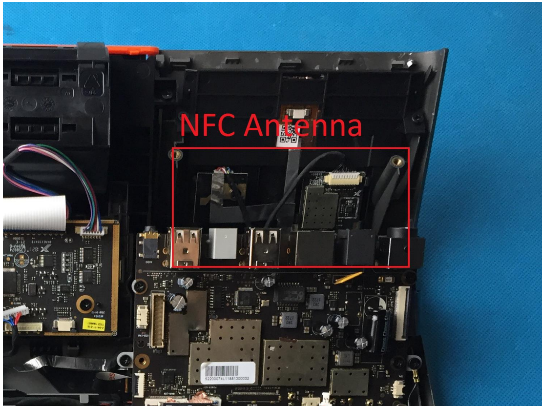
Antenna part
