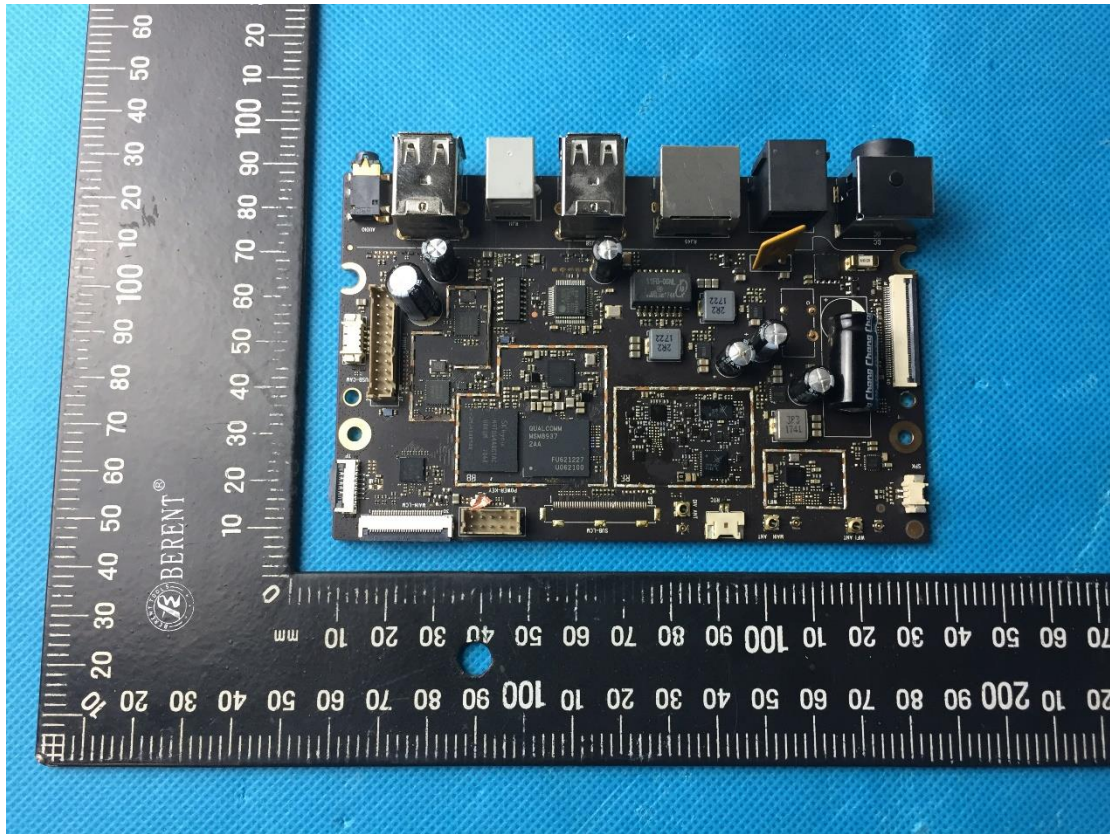
Main board without shielding
