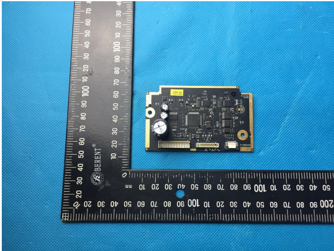
Print Board
