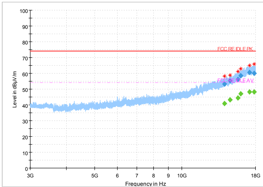
Fig.28 Radiated emission: CH39, 3GHz~18GHz
