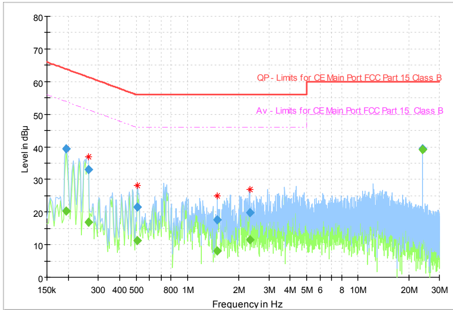
Fig.31 AC Powerline Conducted Emission
