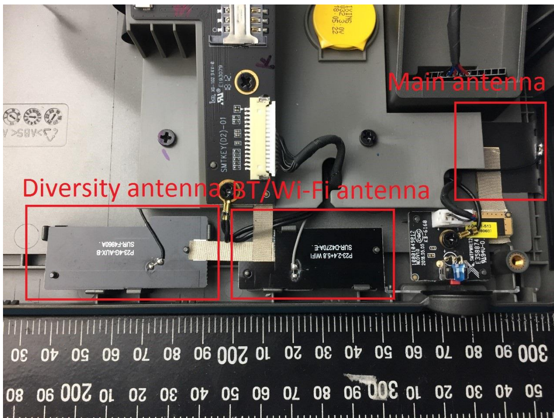
Antenna part
