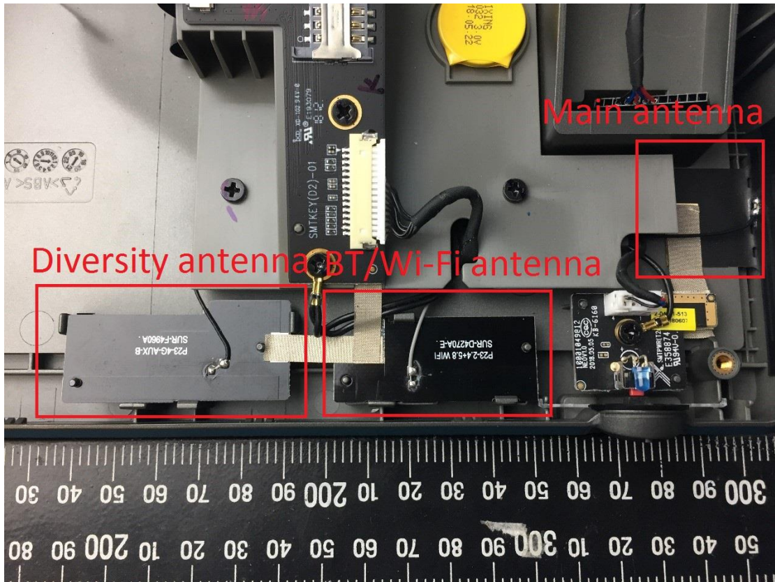
Antenna part
