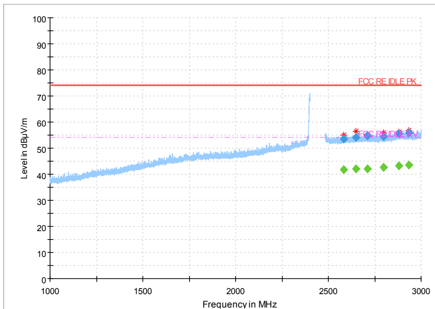
Fig 65. Radiated Spurious Emission (802.11b, Ch1,1GHz~3GHz)
