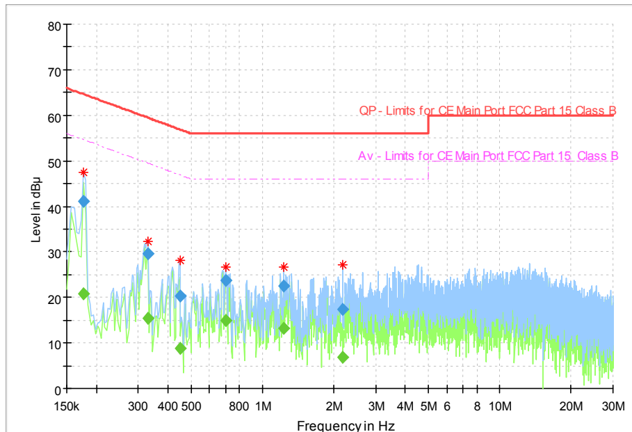
Fig 68. AC Powerline Conducted Emission
