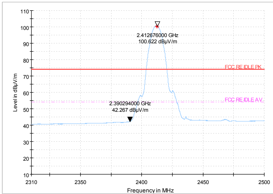
Fig 62. Radiated emission (Power): 802.11b, low channel
