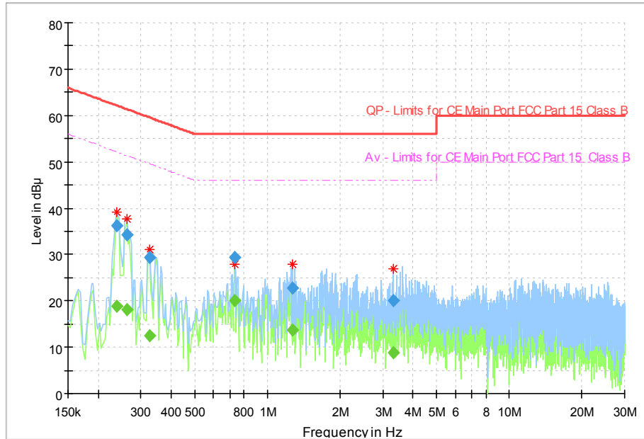
Fig 67. AC Powerline Conducted Emission
