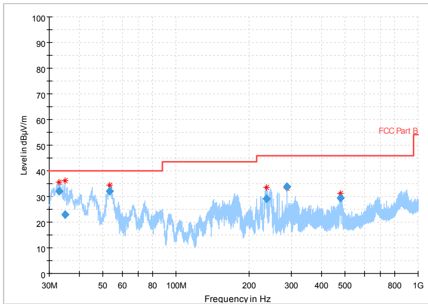
Fig.18 Radiated emission: CH39, 30MHz~1GHz
