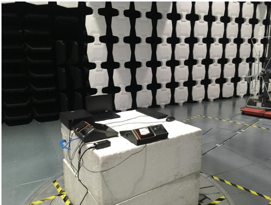
Description: Backview of Radiated Emission Test Setup
