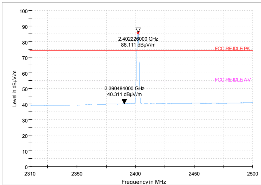
Fig.43 Radiated emission (Low): \pi/4 DQPSK, low channel
