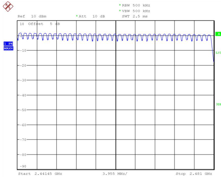
Fig.80 Number of hopping frequency: GFSK, Ch0~39
