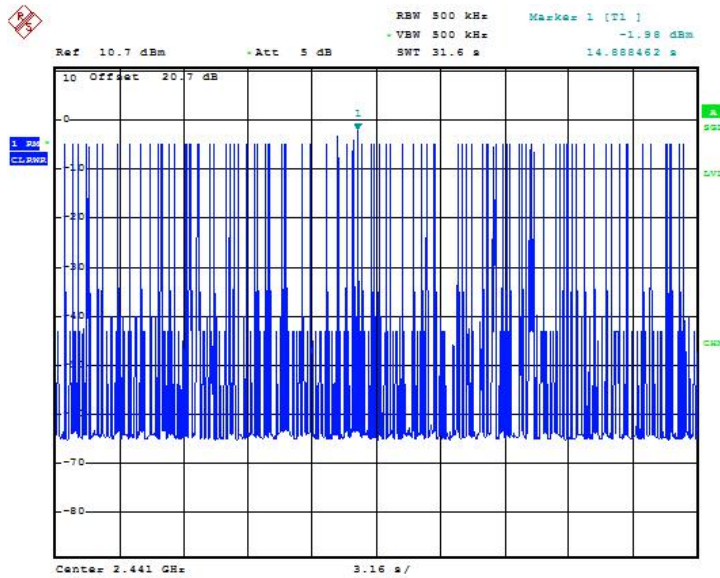
Fig.54 Time of occupancy (Dwell Time): Ch39,Packet DH5
