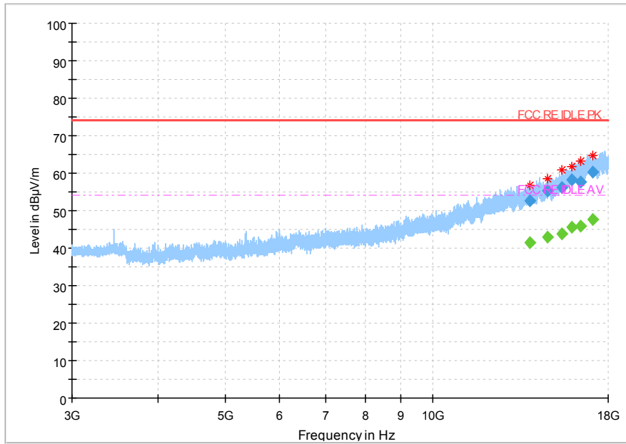
Fig 76. Radiated Spurious Emission (802.11 n-40MHz, Ch3, 3GHz~18GHz) T3521
