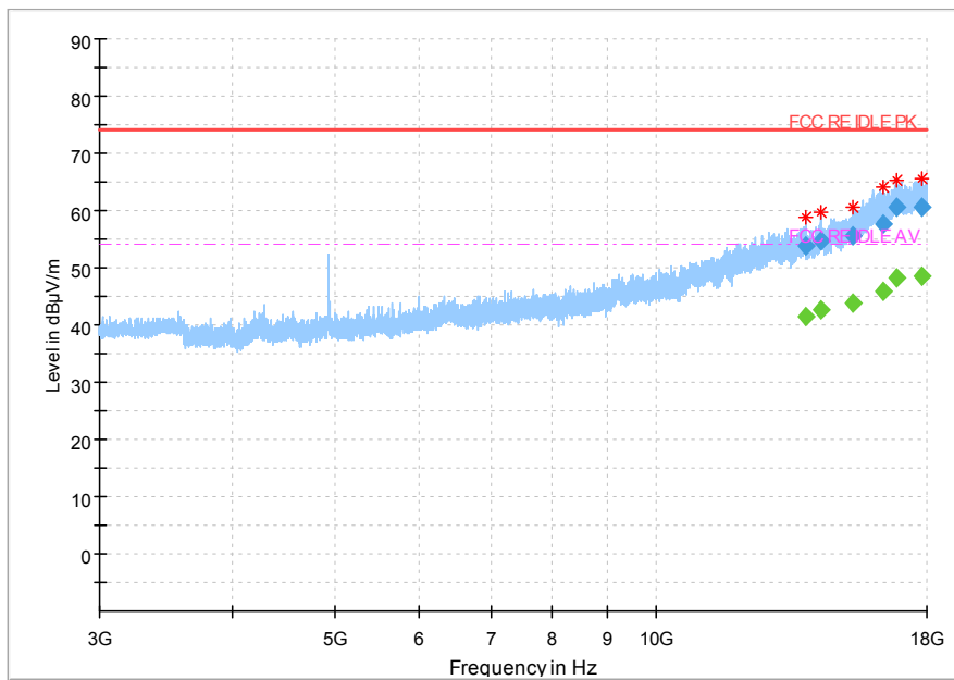
Fig 81. Radiated Spurious Emission (802.11b,Ch11,3GHz~18GHz)
