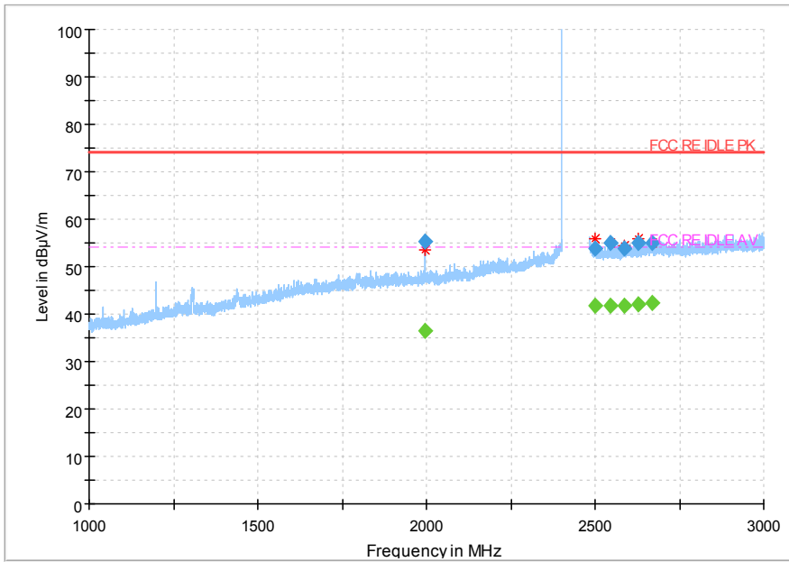
Fig.28 Radiated emission: Ch0, 1GHz~3GHz
