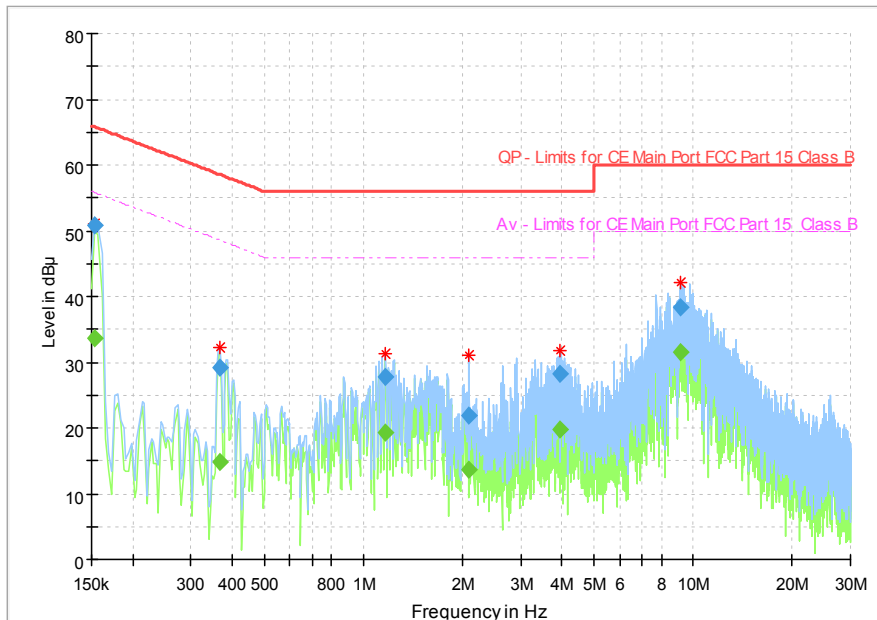
Fig.30 AC Powerline Conducted Emission
