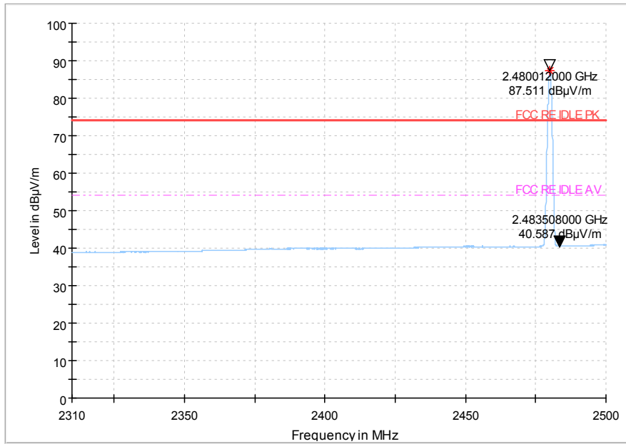
Fig.64 Radiated emission (Power): GFSK, high channel
