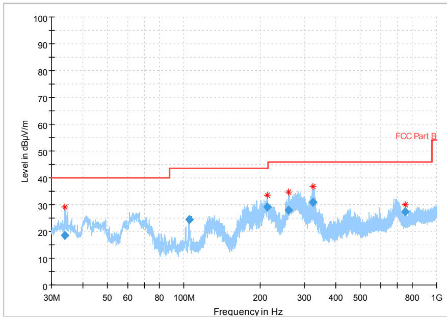
Fig.67 Radiated Spurious Emission (802.11b,Ch11,30MHz~1GHz)
