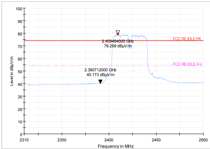
Fig.80 Radiated emission (Power): 802.11n (40M) , low channel
