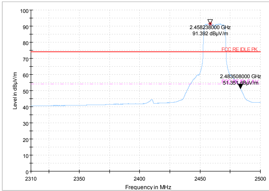
Fig.76 Radiated emission (Power): 802.11n, high channel
