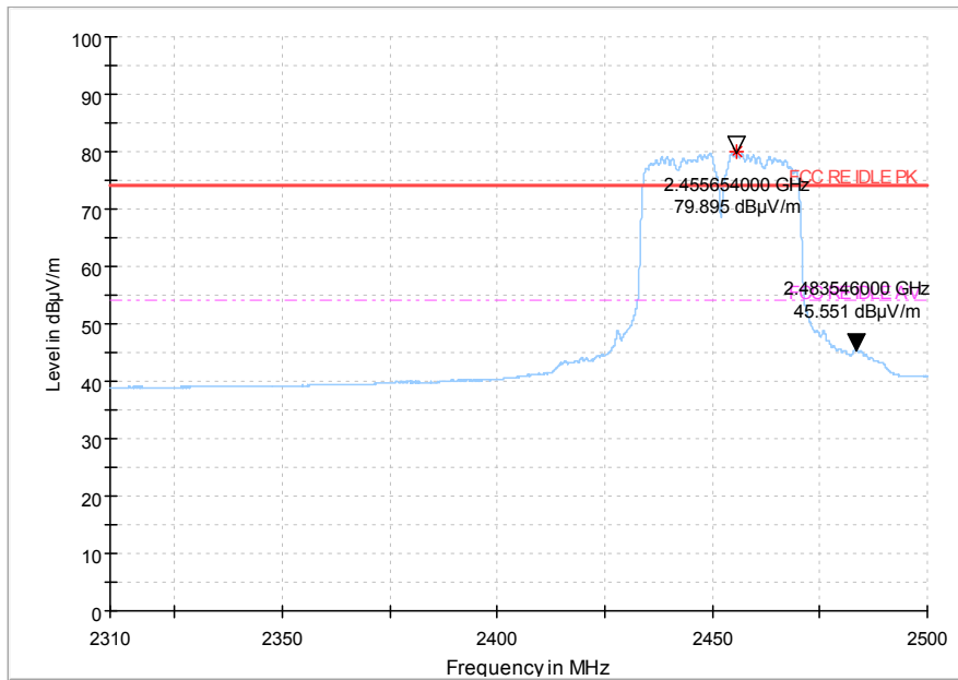
Fig.81 Radiated emission (Power): 802.11n (40M) , high channel
