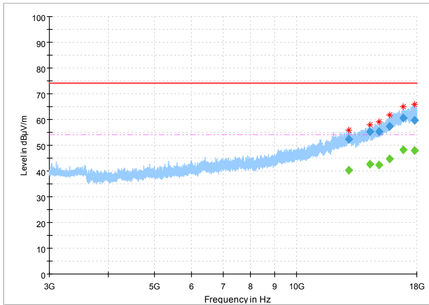
Fig.69 Radiated Spurious Emission (802.11b,Ch11,3GHz~18GHz)
