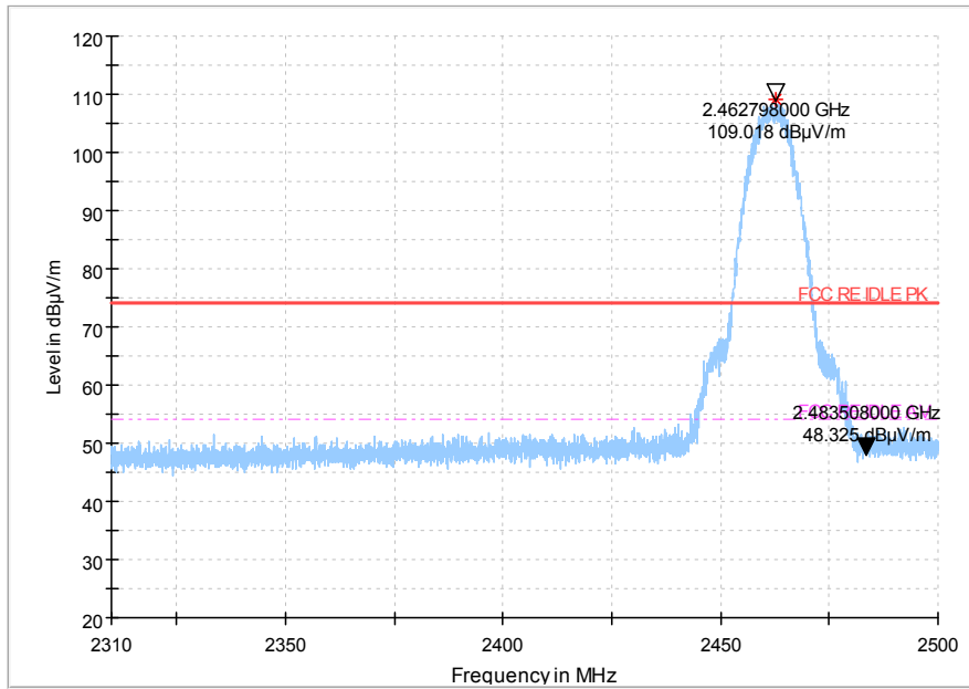
Fig.66 Radiated emission (Power): 802.11b, high channel
