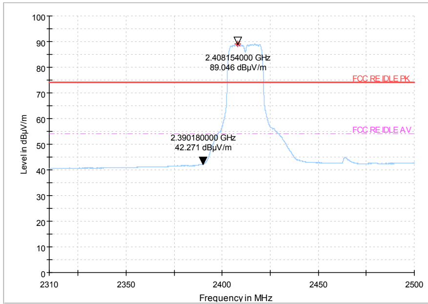
Fig.75 Radiated emission (Power): 802.11n, low channel
