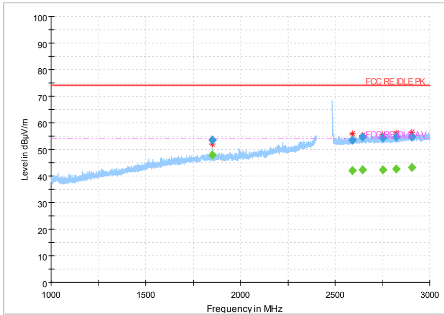
Fig.78 Radiated Spurious Emission (802.11 n-20MHz,Ch11,1GHz~3GHz)
