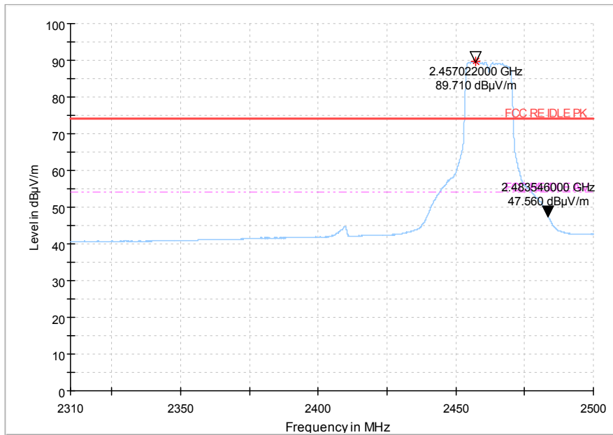
Fig.71 Radiated emission (Power): 802.11g, high channel
