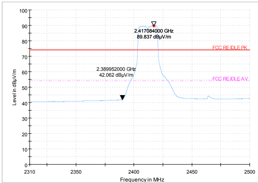
Fig.70 Radiated emission (Power): 802.11g, low channel
