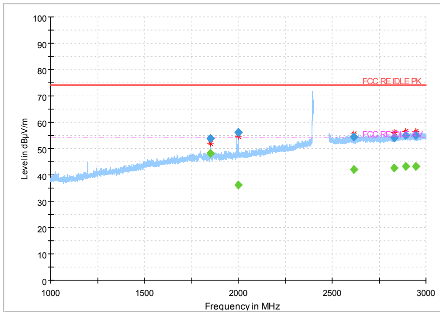
Fig.83 Radiated Spurious Emission (802.11 n-40MHz,Ch3,1GHz~3GHz)
