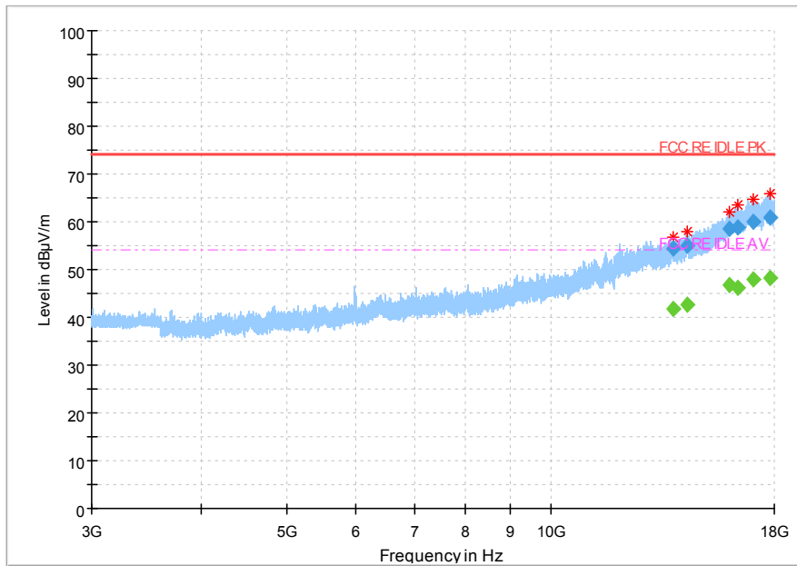
Fig.79 Radiated Spurious Emission (802.11 n-20MHz,Ch11,3GHz~18GHz)
