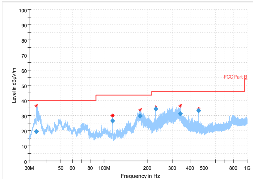
Fig.55 Radiated emission: 8DPSK, Ch0, 30MHz~1GHz
