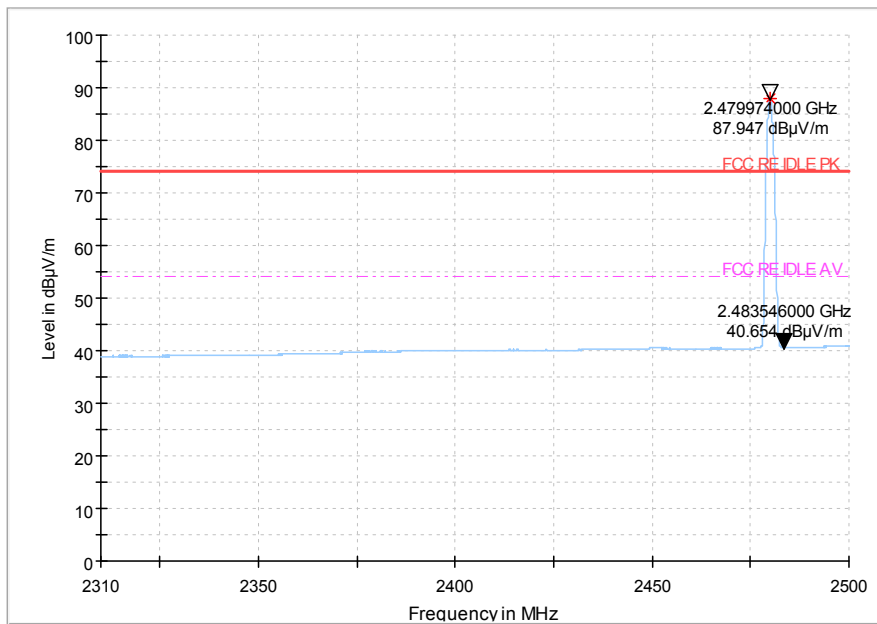
Fig.59 Radiated emission (Power): 8DPSK, high channel
