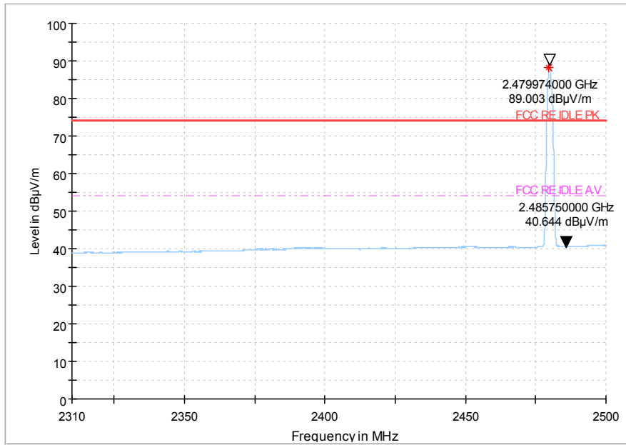
Fig.64 Radiated emission (Power): 8DPSK, high channel
