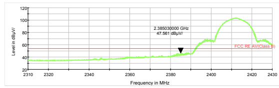
802.11b-Channel 1 Average
