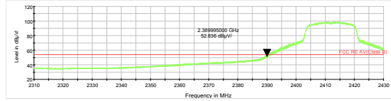
802.11g-Channel 1 Average
