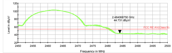
802.11b-Channel 11 Average
