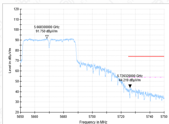
Bandedge-11N(40M)-CH134-AV
