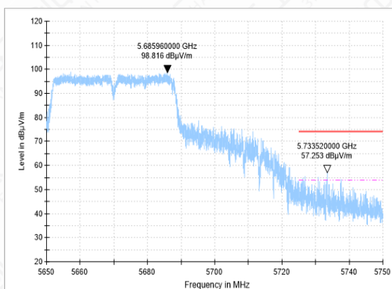
Bandedge-11N(40M)-CH134-PK
