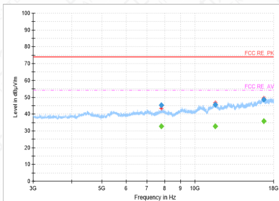
RSE-11N(40M)-CH9-3GHz-18GHz
