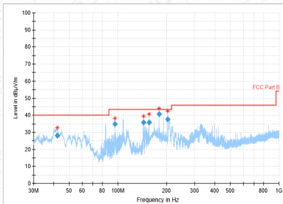
RSE-11N(40M)-CH9-30MHz-1GHz
