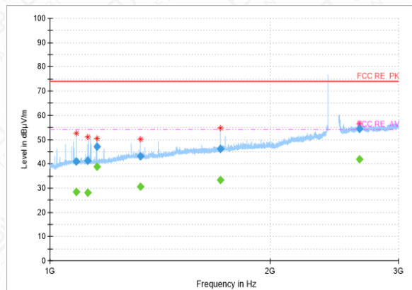
RSE-11N(40M)-CH9-1GHz-3GHz
