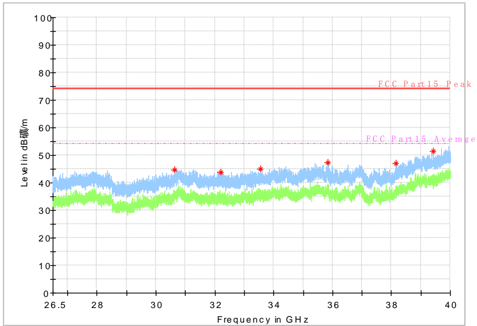
Fig. 30 Radiated emission: 802.11n, (802.11a, Ch149, 26.5 GHz - 40 GHz)
