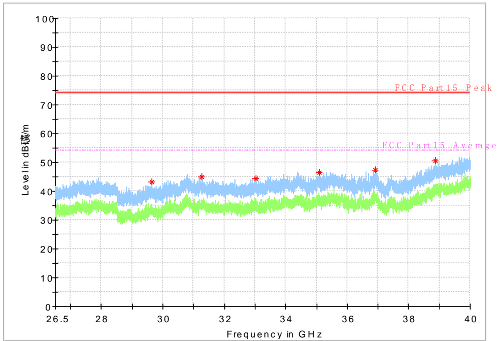
Fig. 46 Radiated emission: 802.11n, (802.11a, Ch149, 26.5 GHz - 40 GHz)
