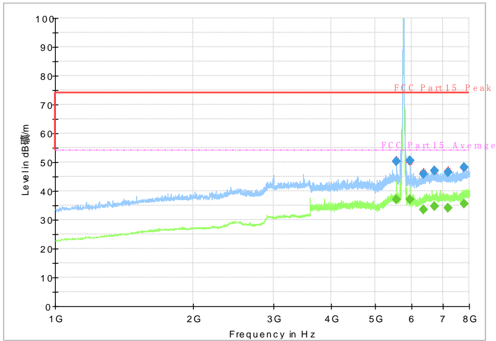
Fig. 48 Radiated Spurious Emission (802.11a, Ch149, 1 GHz-8 GHz)
