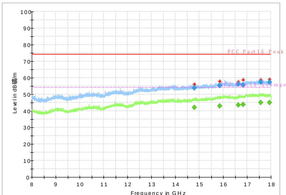
Fig. 53 Radiated Spurious Emission (802.11n-HT40, ch38, 8 GHz-18 GHz)
