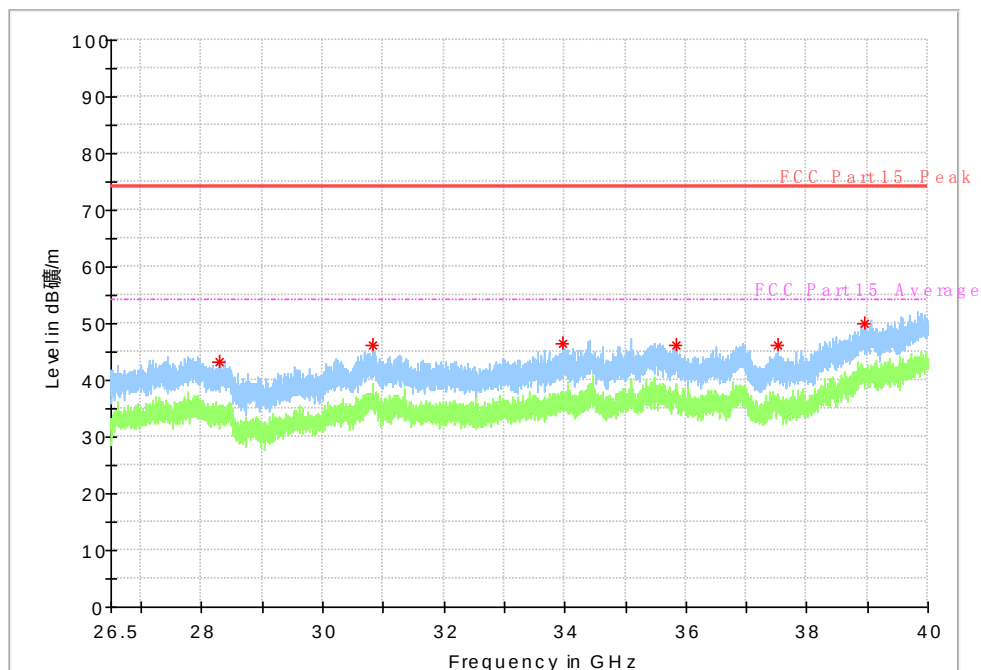
Fig. 45 Radiated Spurious Emission (802.11a, ch36, 26.5 GHz-40 GHz)
