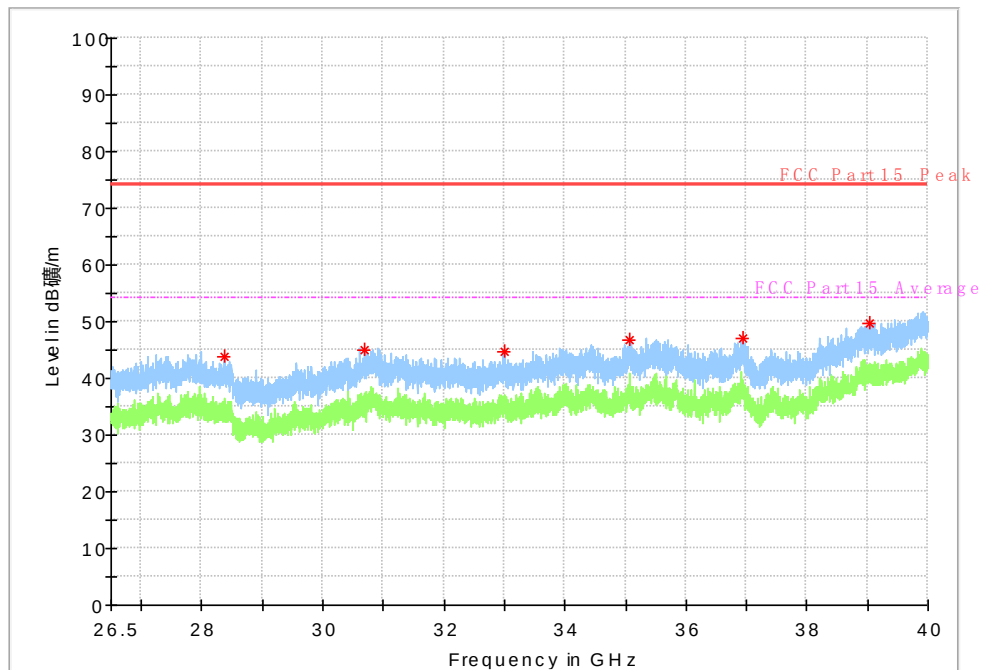
Fig. 55 Radiated Spurious Emission (802.11n-HT40, ch38, 26.5 GHz-40 GHz)
