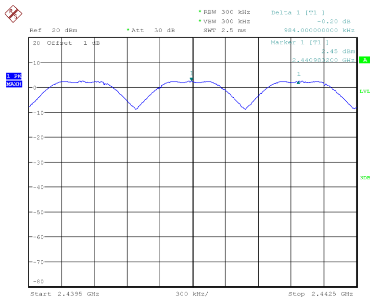
Fig.92 Carrier separation measurement: GFSK, Ch39
