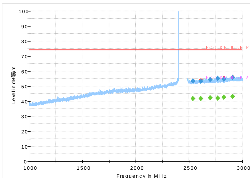
Fig.56 Radiated emission: GFSK, Ch0, 1GHz~3GHz
