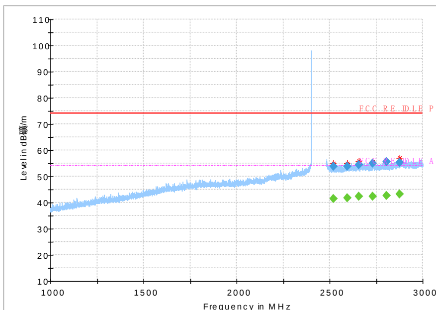
Fig.61 Radiated emission: GFSK, Ch0, 1GHz~3GHz
