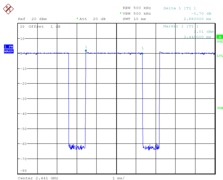
Fig.74 Number of Transmissions Measurement: Ch39, Packet 2-DH3
