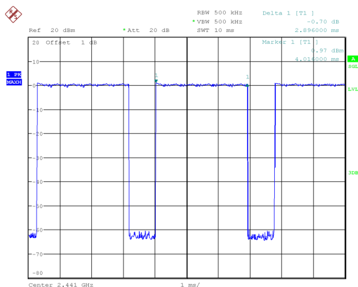
Fig.80 Number of Transmissions Measurement: Ch39, Packet 3-DH3
