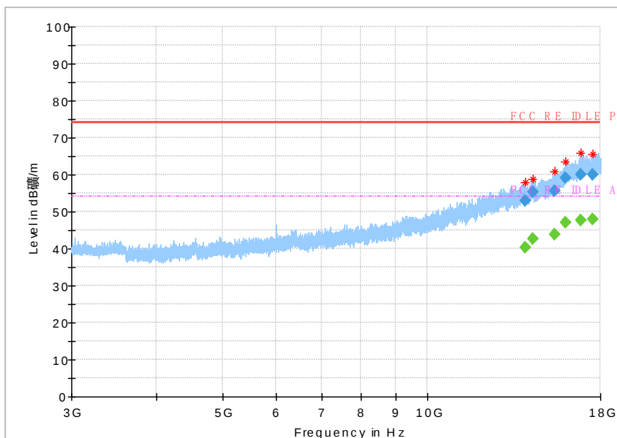
Fig.57 Radiated emission: GFSK, Ch0, 3GHz~18GHz
