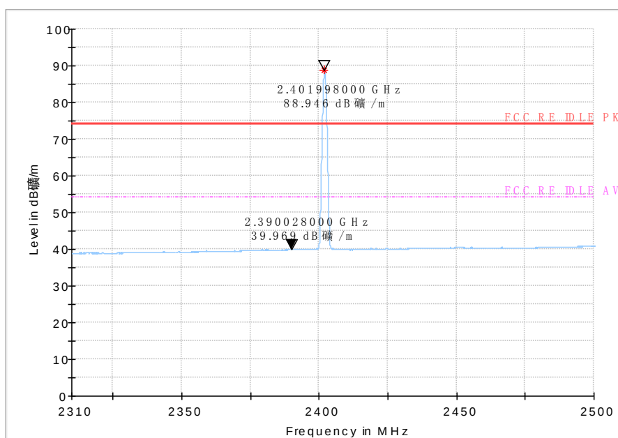
Fig.58 Radiated emission (Low): GFSK, low channel
