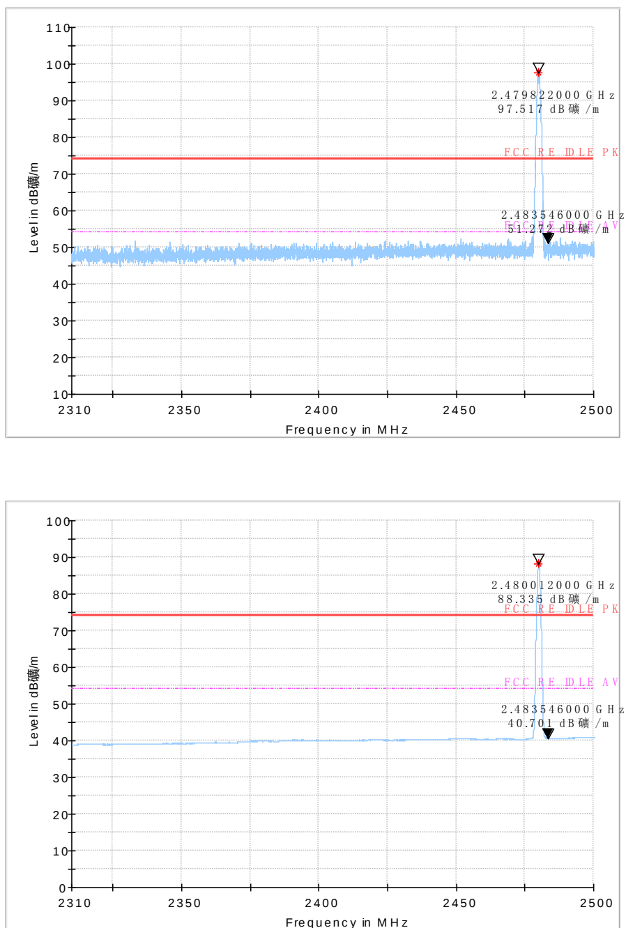
Fig.59 Radiated emission (High): GFSK, high channel
