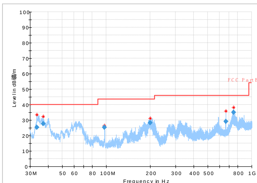
Fig.55 Radiated emission: GFSK, Ch0, 30MHz~1GHz
