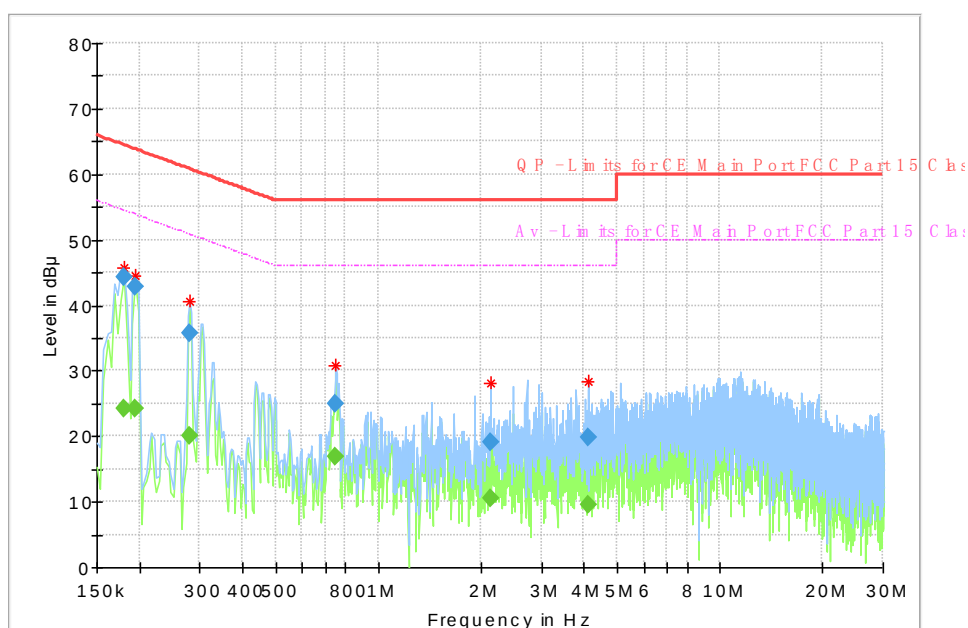
Fig.102 AC Powerline Conducted Emission
