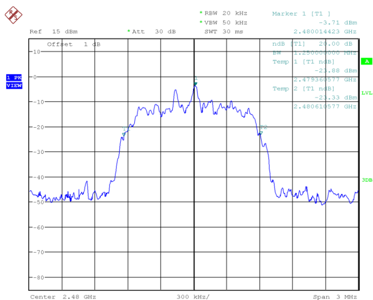
Fig.84 20dB Bandwidth: GFSK, Ch39
