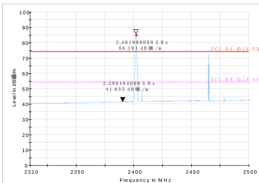
Fig.63 Radiated emission (Low): GFSK, low channel
