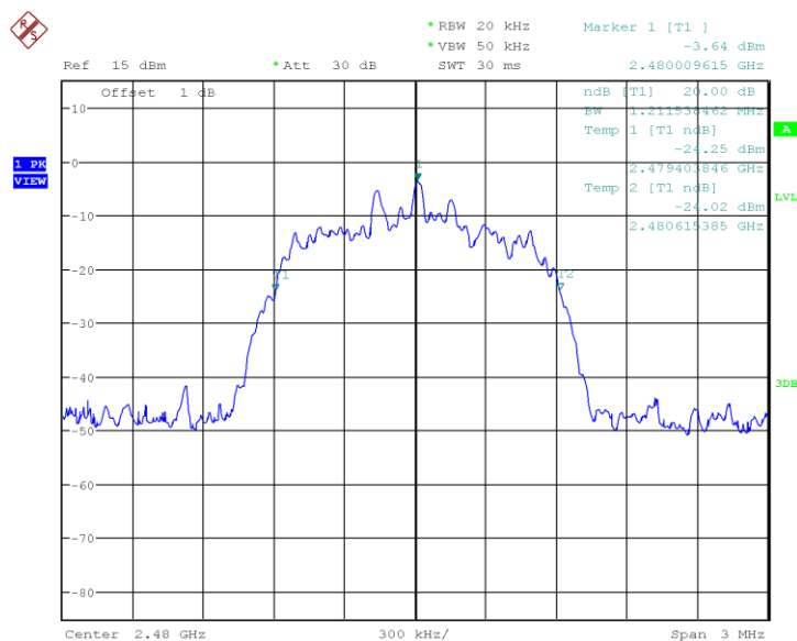
Fig.90 20dB Bandwidth: 8DPSK, Ch39
