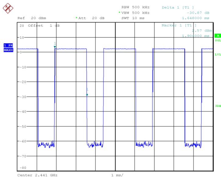
Fig.66 Number of Transmissions Measurement: Ch39, Packet DH1
