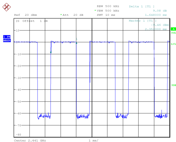
Fig.72 Number of Transmissions Measurement: Ch39, Packet 2-DH1
