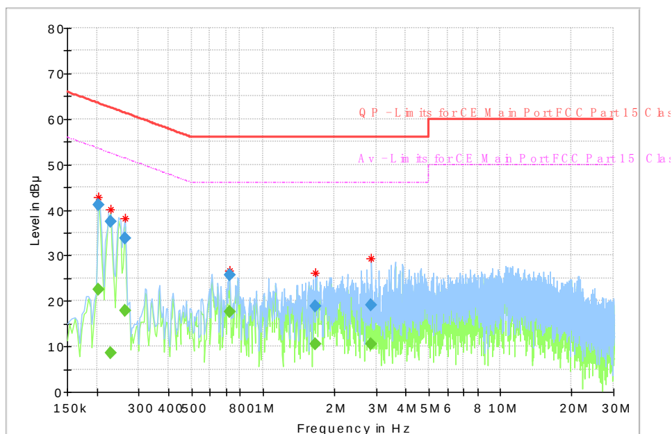
Fig.101 AC Powerline Conducted Emission
