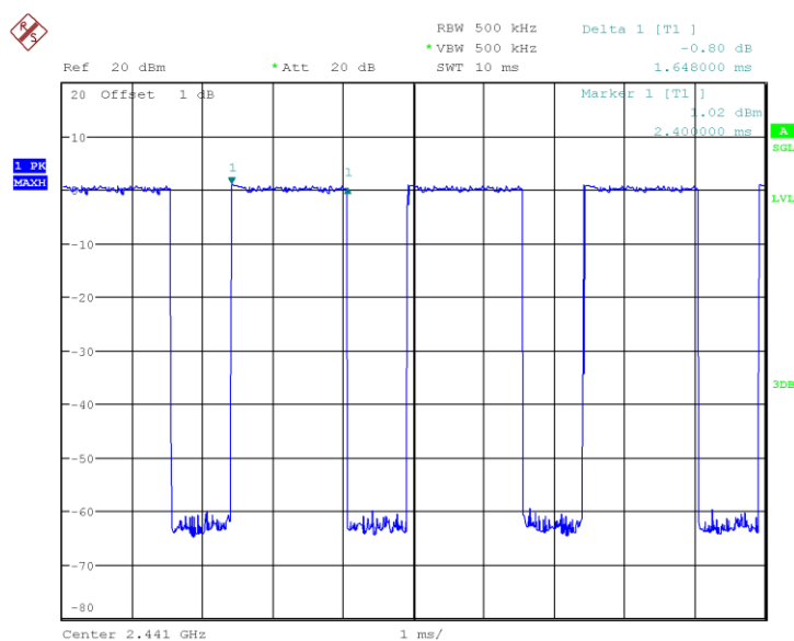
Fig.78 Number of Transmissions Measurement: Ch39, Packet 3-DH1
