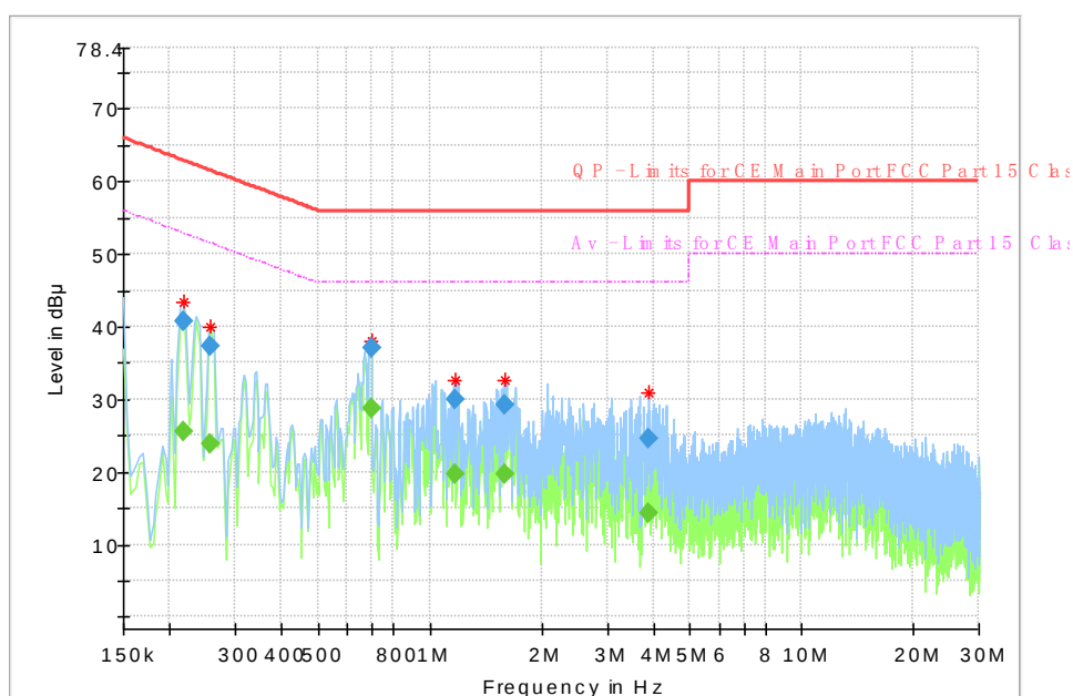
Fig.103 AC Powerline Conducted Emission
