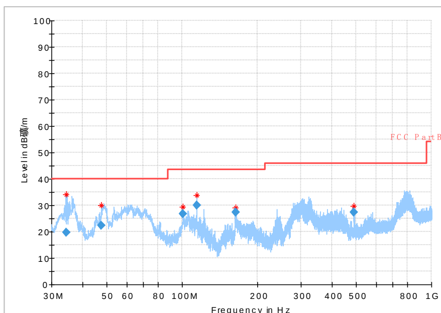
Fig.60 Radiated emission: GFSK, Ch0, 30MHz~1GHz
