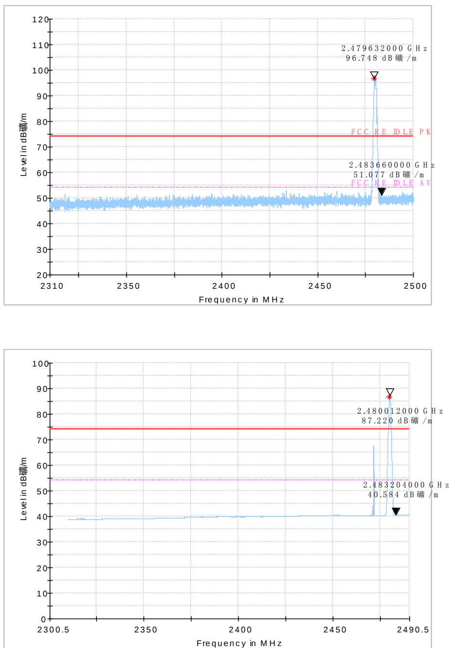
Fig.64 Radiated emission (High): GFSK, high channel
