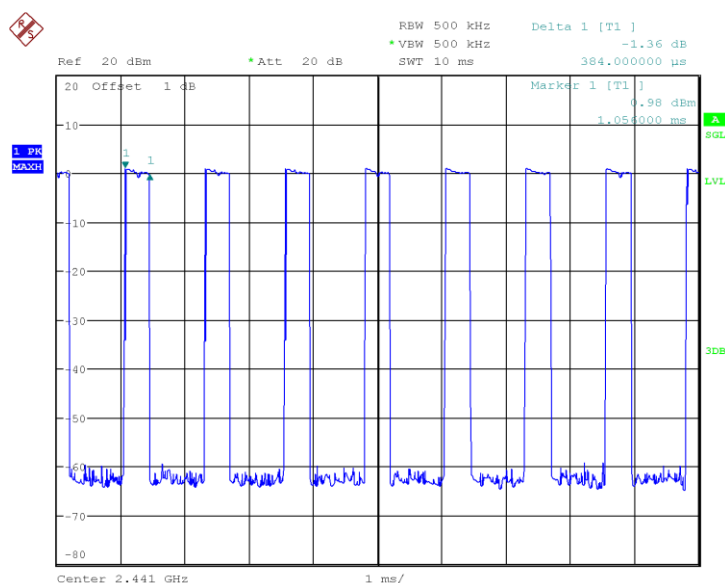
Fig.70 Number of Transmissions Measurement: Ch39, Packet DH5
