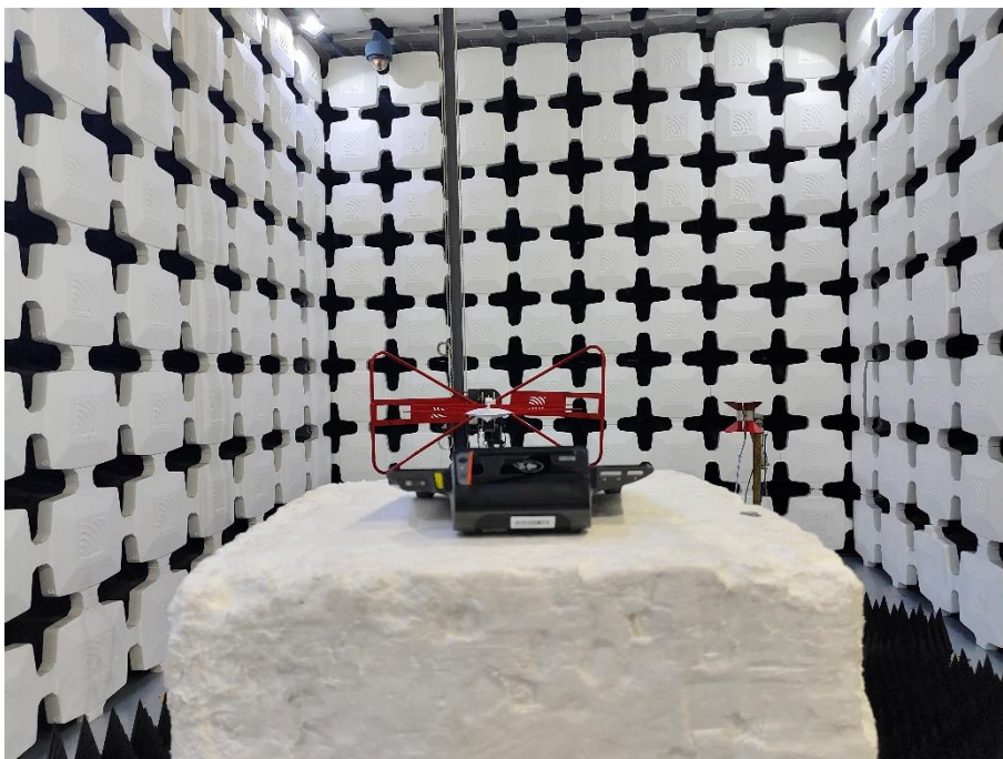
10. Radiated Emissions (Part 22/24/27, 30MHz-18GHz)
