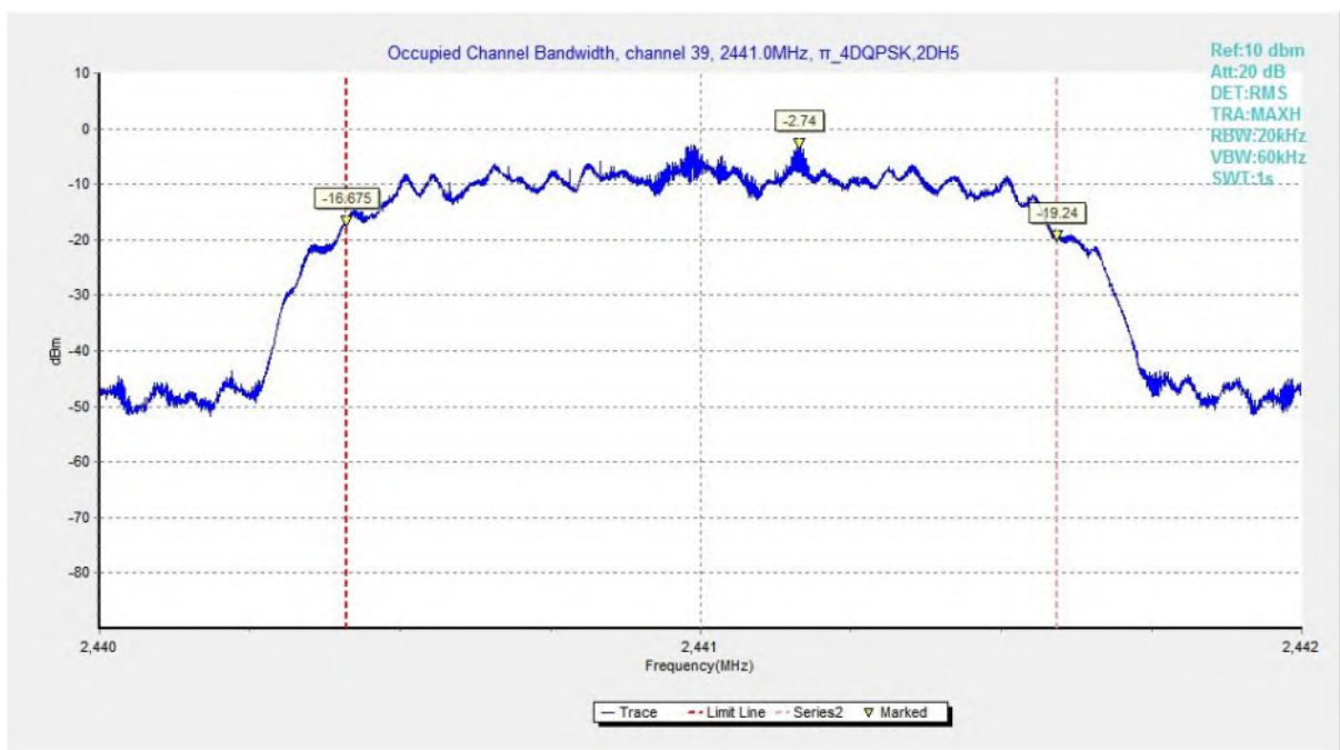
Fig. 81 99% Occupied Bandwidth ( \pi /4 DQPSK, Ch 39)
