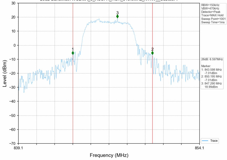
26dB Bandwidth WCDMA_5_HSUPA_HCH_846.6MHz_NTNV__Subtest 1
