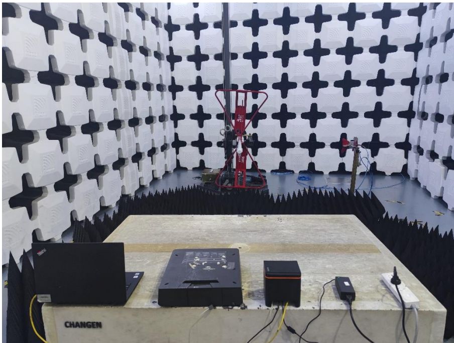
2. Radiated Emissions (Part 15B Data Transfer/Print,1GHz-18GHz)
