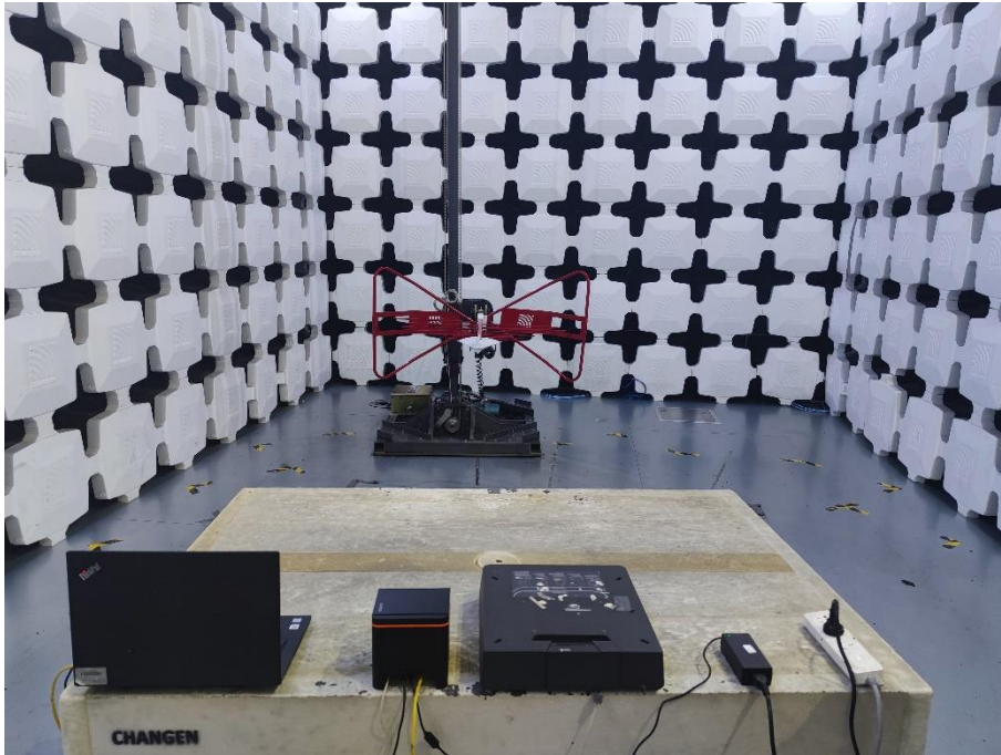
1. Radiated Emissions (Part 15B Data Transfer/Print,30MHz-1GHz)
