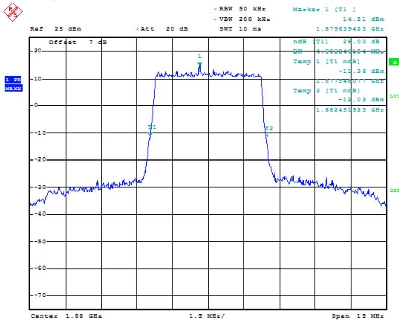
Fig.41 LTE band 2, 5MHz Bandwidth, QPSK (-26dBc BW)
