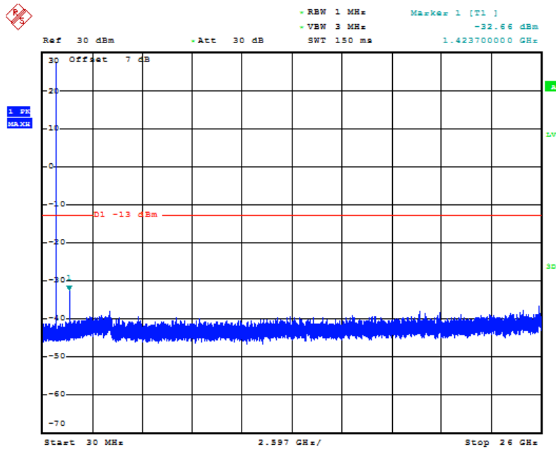
Fig.91 LTE band 7: 30MHz – 26GHz
