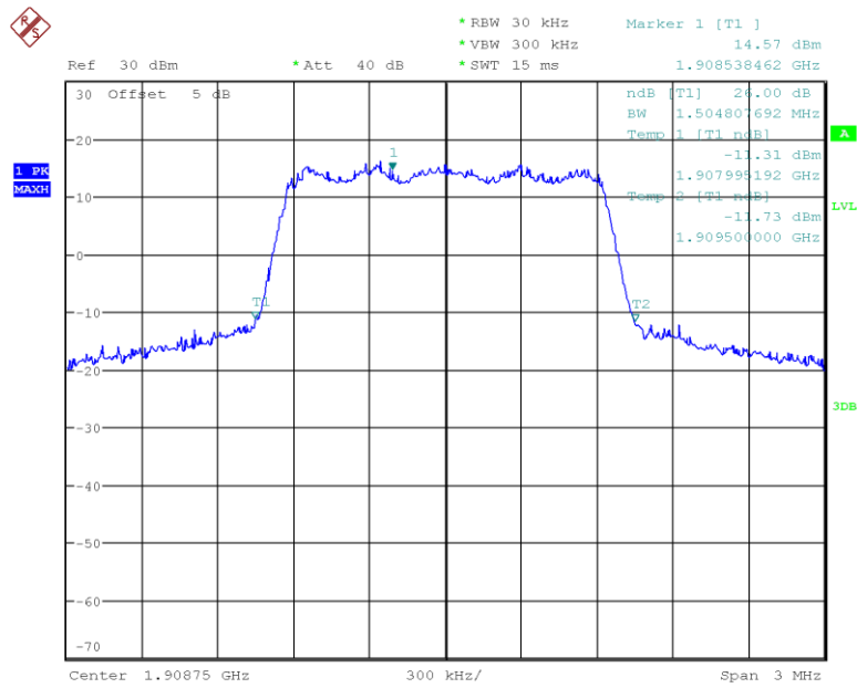
Fig.24 Channel 1175- Emission Bandwidth (-26dBc BW)
