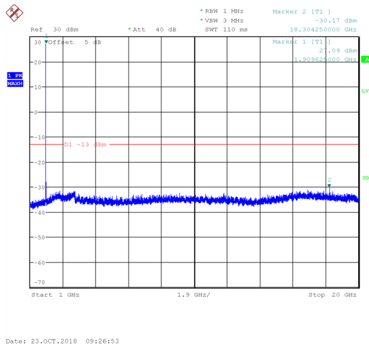
Fig.68 Channel 810: 1GHz~20GHz
