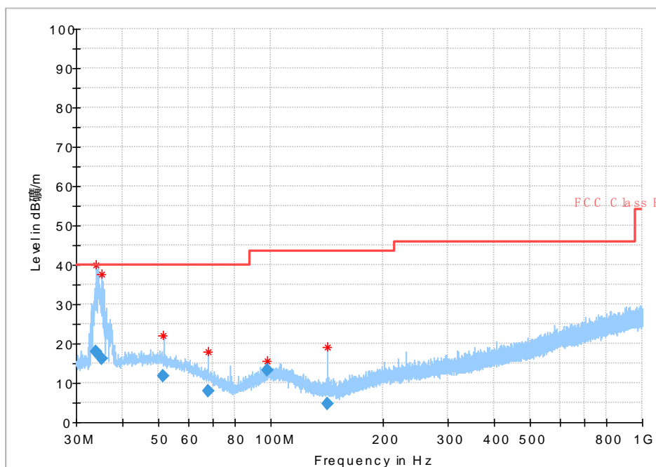
Fig. 26 Radiated Spurious Emission (802.11a, Ch149, 30 MHz-1 GHz)
