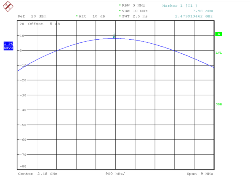
Fig.2 Peak Conducted Output Power CH39, DH1
