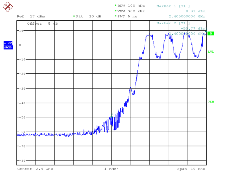
Fig.10 Frequency Band Edge: GFSK, Ch0, Hopping OFF
