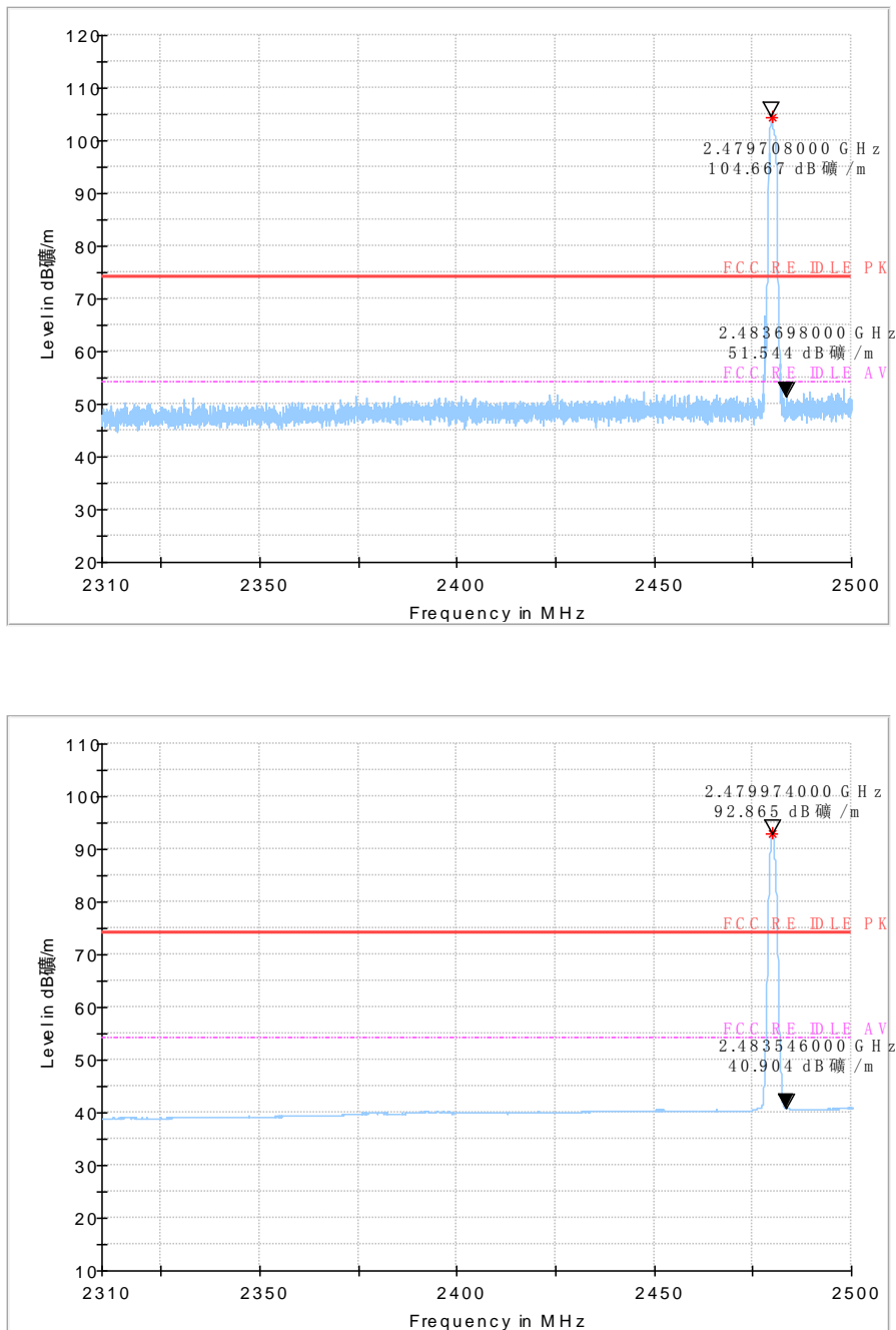
Fig.54 Radiated emission (High): 8DPSK, high channel
