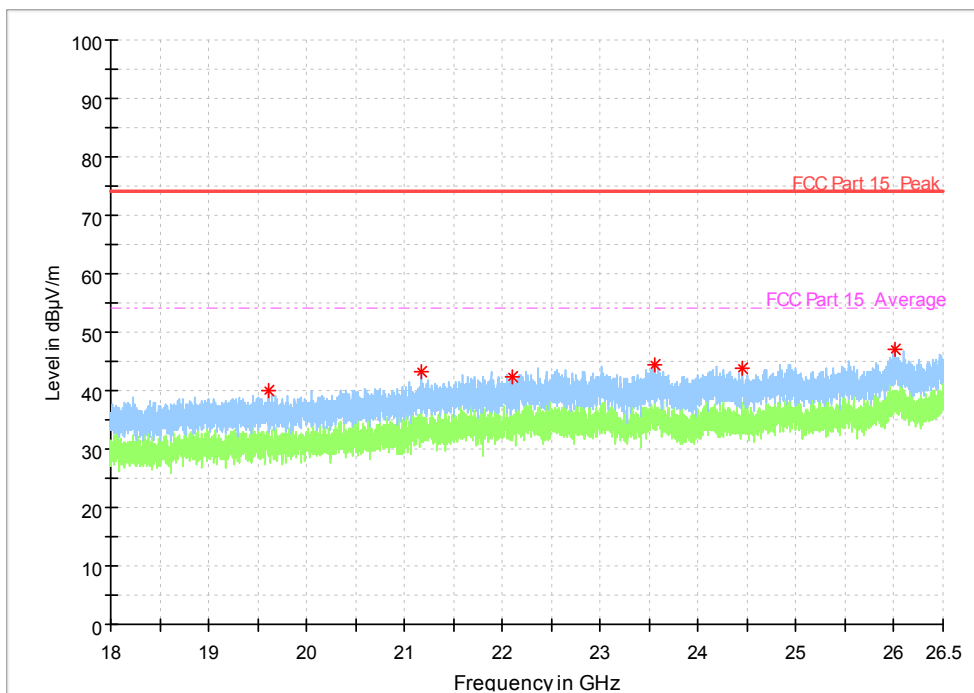
Fig. 26 Radiated Spurious Emission (802.11n-HT20, Ch149, 18 GHz-26.5 GHz)
