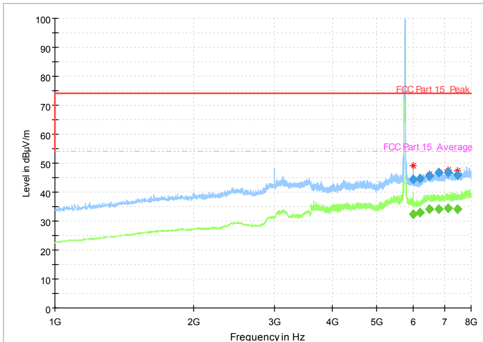
Fig. 24 Radiated Spurious Emission (802.11n-HT20, Ch149, 1 GHz-8 GHz)
