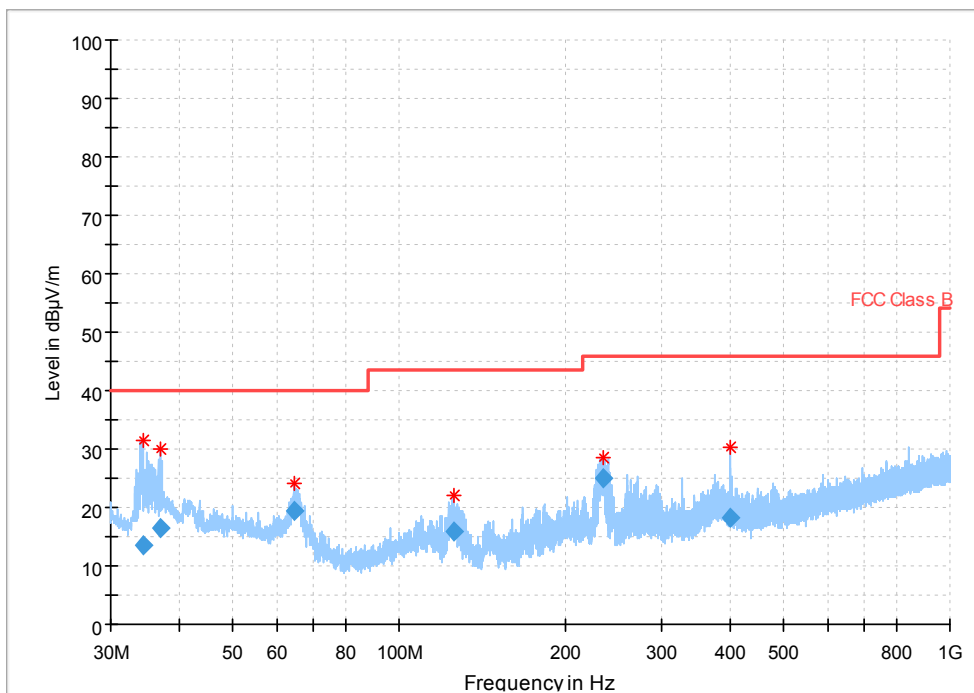
Fig. 28 Radiated Spurious Emission (802.11n-HT40, Ch151, 30 MHz-1 GHz)
