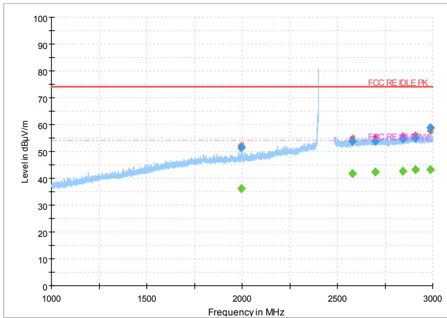
Fig.105 Radiated Spurious Emission (802.11g,Ch1,1GHz~3GHz)
