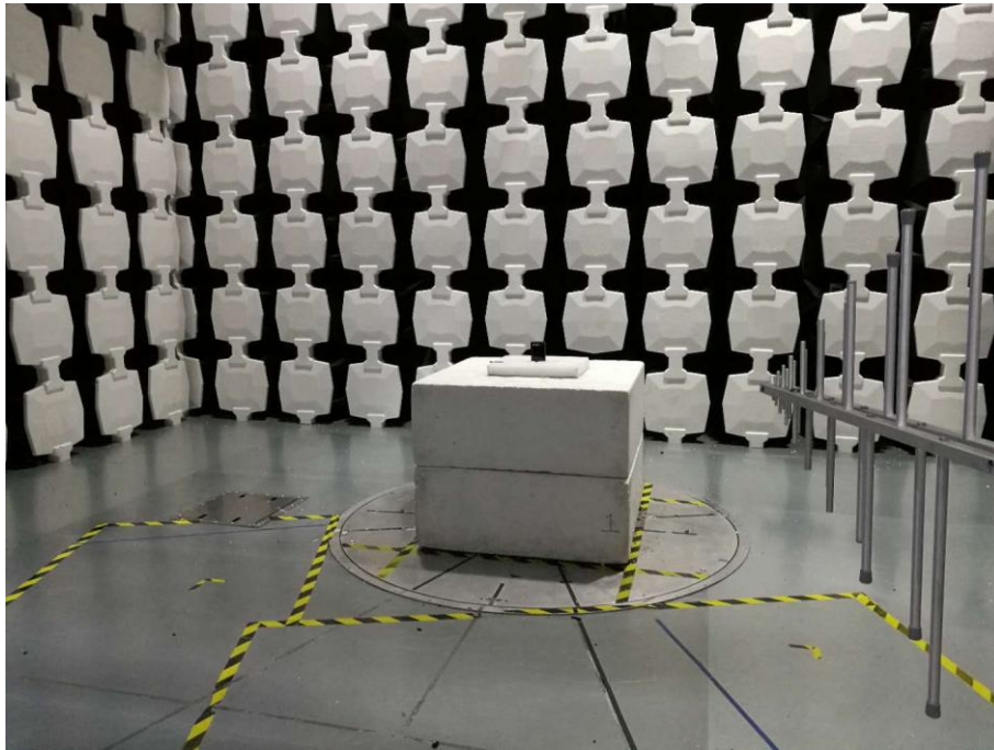
Description: Radiated Emission Test Setup (Above 30MHz)
