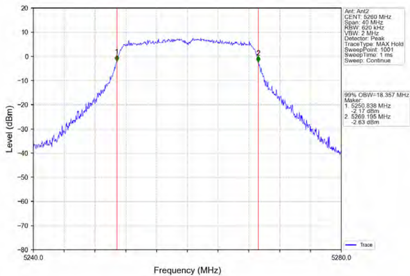
802.11ac(VHT20)_LCH_5260MHz_Ant2_NTNV
