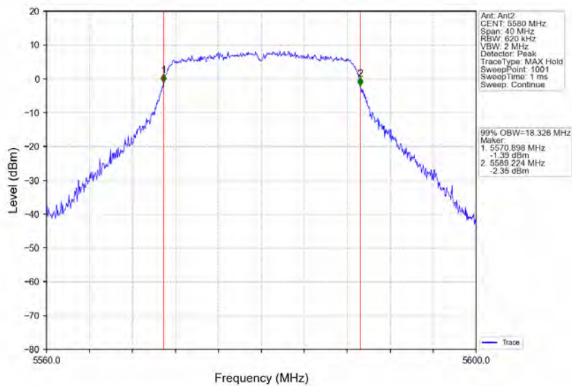
802.11ac(VHT20)_MCH_5580MHz_Ant2_NTNV
