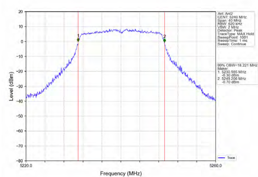
802.11n(HT20)_HCH_5240MHz_Ant2_NTNV
