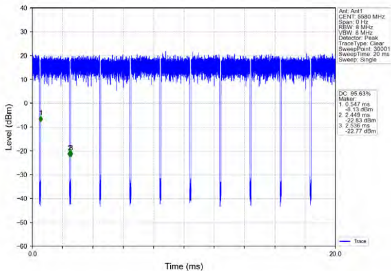
802.11ac(VHT20)_MCH_5580MHz_Ant1_NTNV
