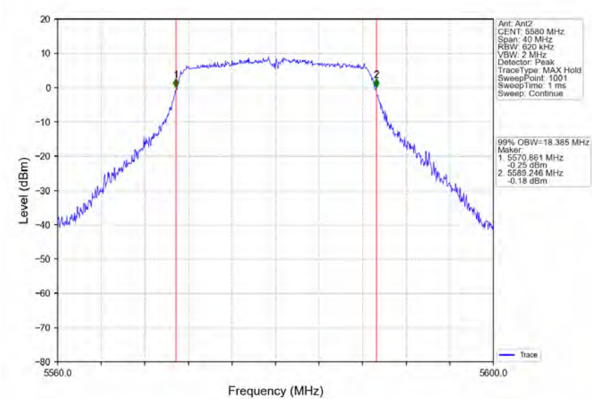
802.11n(HT20)_MCH_5580MHz_Ant2_NTNV
