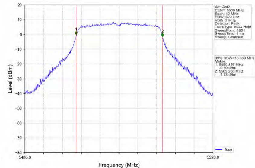
802.11ac(VHT20)_LCH_5500MHz_Ant2_NTNV
