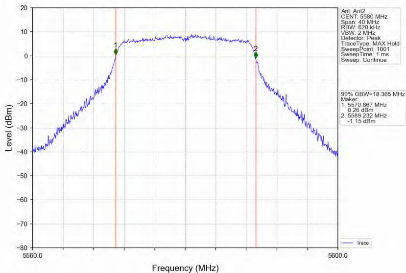
802.11n(HT20)_MCH_5580MHz_Ant2_NTNV
