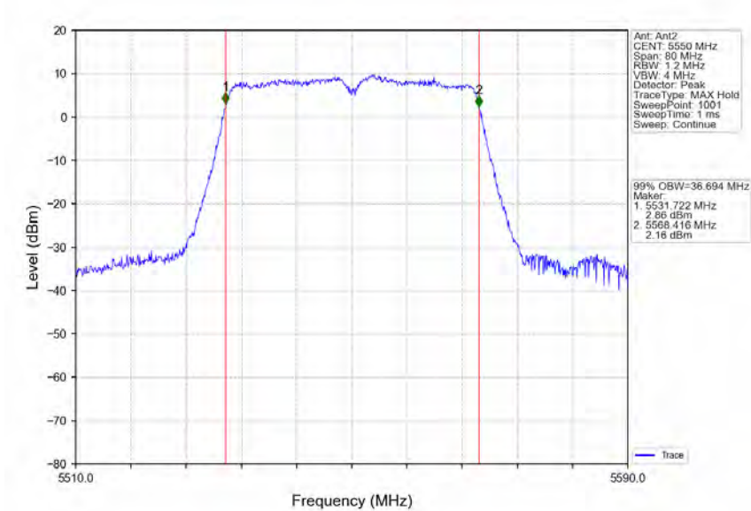
802.11n(HT40)_MCH_5550MHz_Ant2_NTNV
