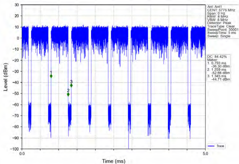
802.11ac(VHT80)_MCH_5775MHz_Ant1_NTNV
