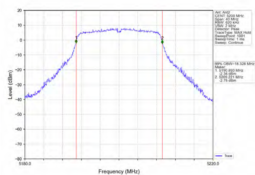
802.11ac(VHT20)_MCH_5200MHz_Ant2_NTNV
