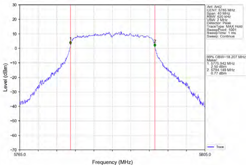
802.11ac(VHT20)_MCH_5785MHz_Ant2_NTNV
