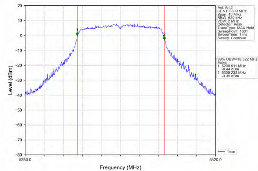
802.11ac(VHT20)_MCH_5300MHz_Ant2_NTNV
