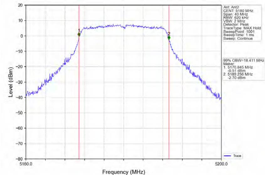
802.11ac(VHT20)_LCH_5180MHz_Ant2_NTNV
