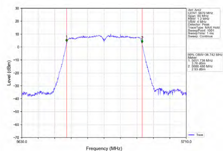
802.11n(HT40)_HCH_5670MHz_Ant2_NTNV
