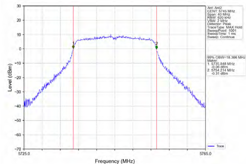
802.11n(HT20)_LCH_5745MHz_Ant2_NTNV
