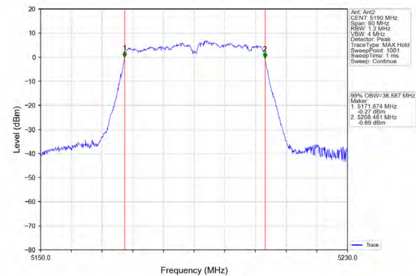
802.11ac(VHT40)_LCH_5190MHz_Ant2_NTNV
