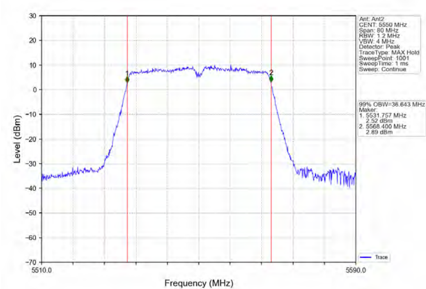
802.11n(HT40)_MCH_5550MHz_Ant2_NTNV
