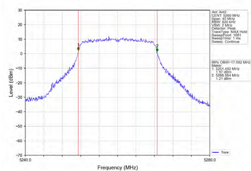
802.11a_LCH_5260MHz_Ant2_NTNV
