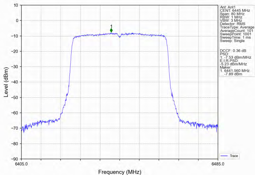
802.11ax(HEW40)_LCH_6445MHz_RU484_Left_Ant1_NTNV
