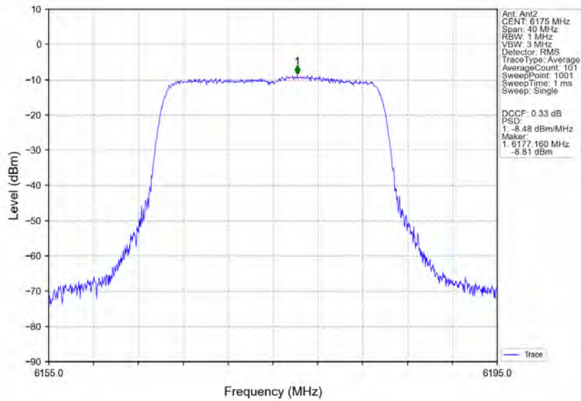
802.11ax(HEW20)_MCH_6175MHz_RU242_Left_MIMO_NTNV
