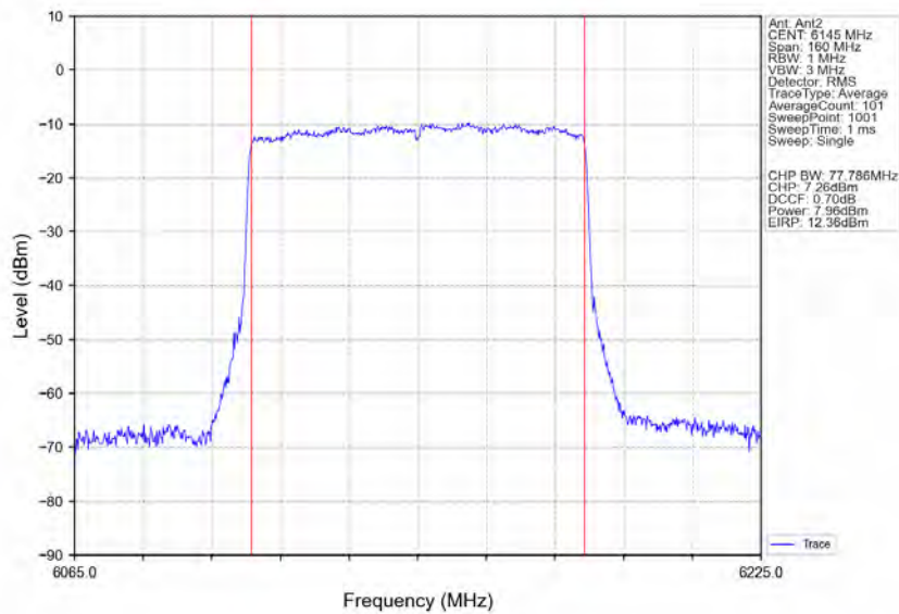
802.11ax(HEW80)_MCH_6145MHz_RU996_Left_Ant2_NTNV
