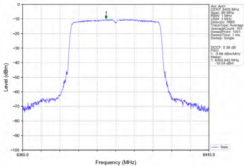
802.11ax(HEW40)_HCH_6405MHz_RU484_Left_Ant1_NTNV
