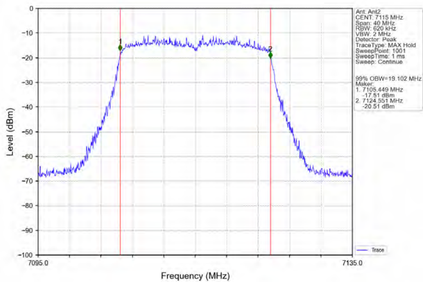
802.11ax(HEW20)_HCH_7115MHz_RU242_Left_Ant2_NTNV
