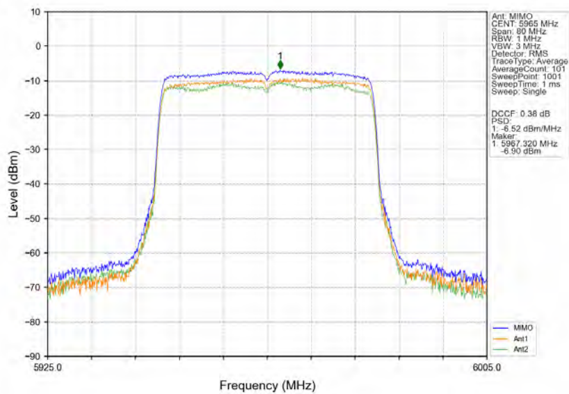
802.11ax(HEW40)_LCH_5965MHz_RU484_Left_MIMO_NTNV
