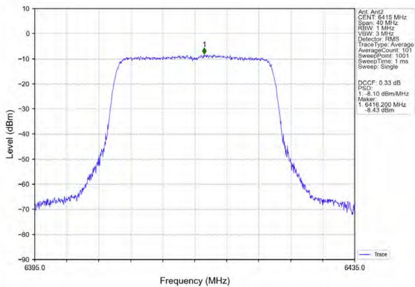
802.11ax(HEW20)_HCH_6415MHz_RU242_Left_Ant2_NTNV
