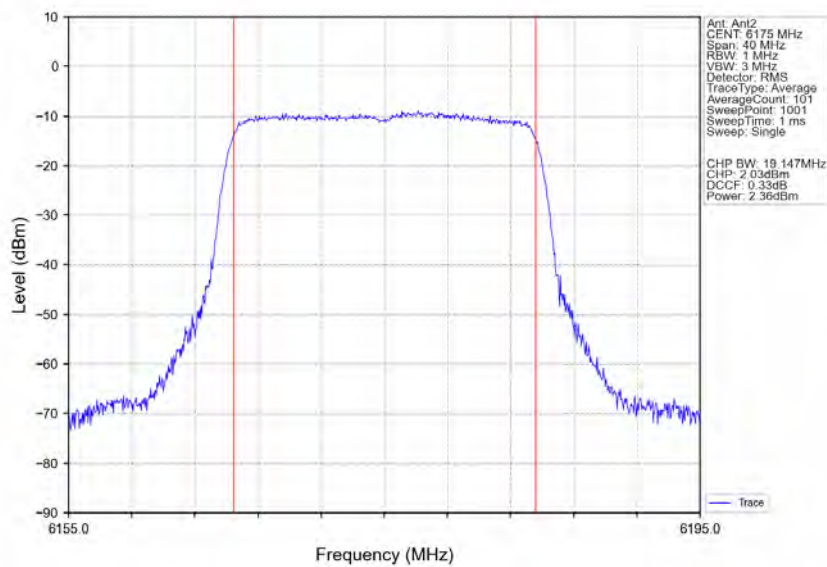
802.11ax(HEW20)_MCH_6175MHz_RU242_Left_Ant2_NTNV
