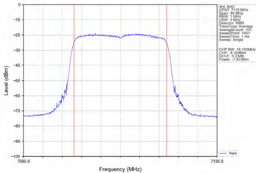
802.11ax(HEW20)_HCH_7115MHz_RU242_Left_Ant2_NTNV
