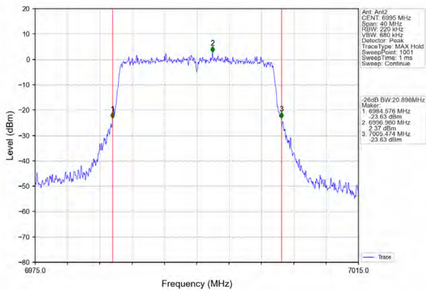
802.11ax(HEW20)_MCH_6995MHz_RU242_Left_Ant2_NTNV
