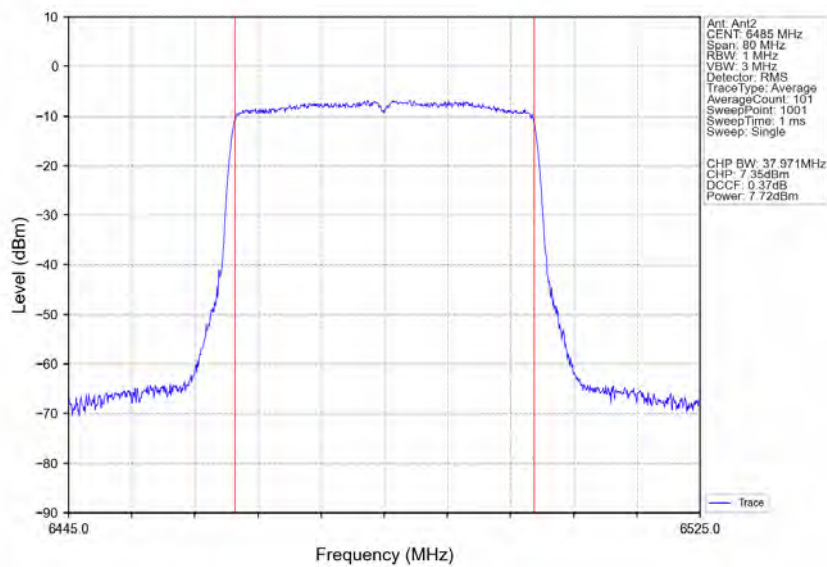
802.11ax(HEW40)_MCH_6485MHz_RU484_Left_Ant2_NTNV
