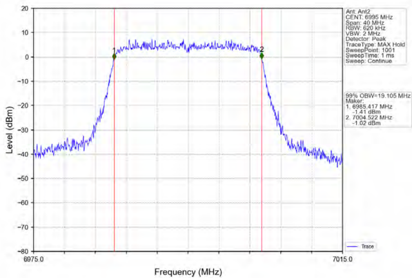
802.11ax(HEW20)_MCH_6995MHz_RU242_Left_Ant2_NTNV
