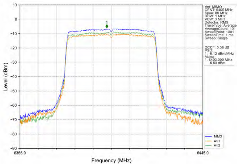
802.11ax(HEW40)_HCH_6405MHz_RU484_Left_MIMO_NTNV
