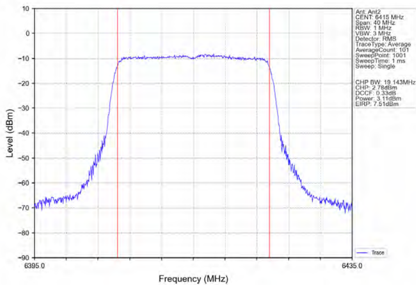
802.11ax(HEW20)_HCH_6415MHz_RU242_Left_Ant2_NTNV
