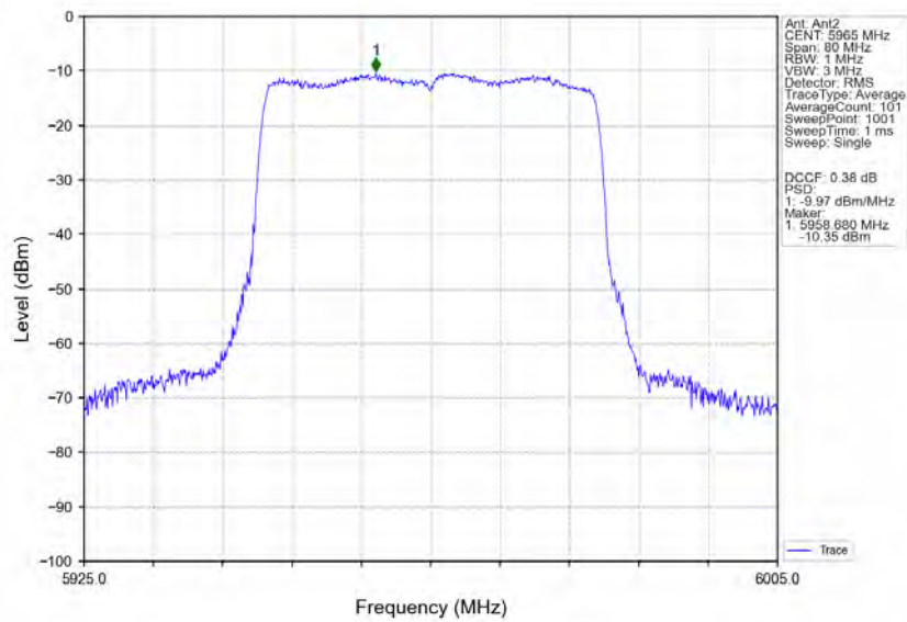
802.11ax(HEW40)_LCH_5965MHz_RU484_Left_MIMO_NTNV
