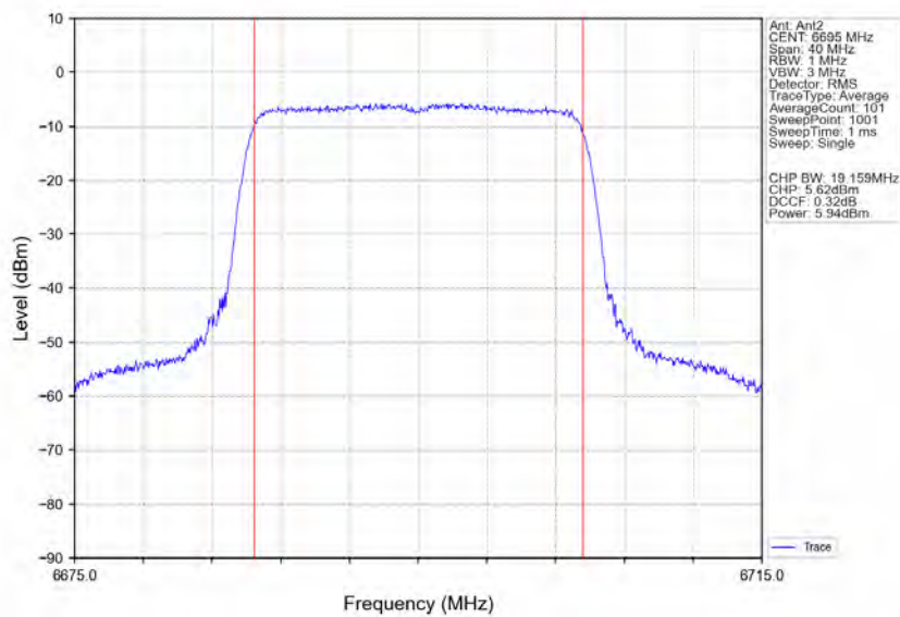
802.11ax(HEW20)_MCH_6695MHz_RU242_Left_Ant2_NTNV
