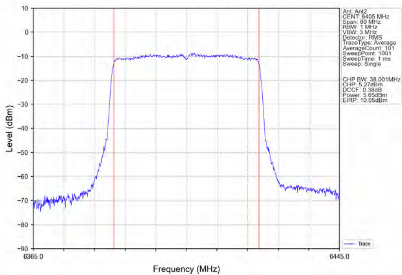
802.11ax(HEW40)_HCH_6405MHz_RU484_Left_Ant2_NTNV
