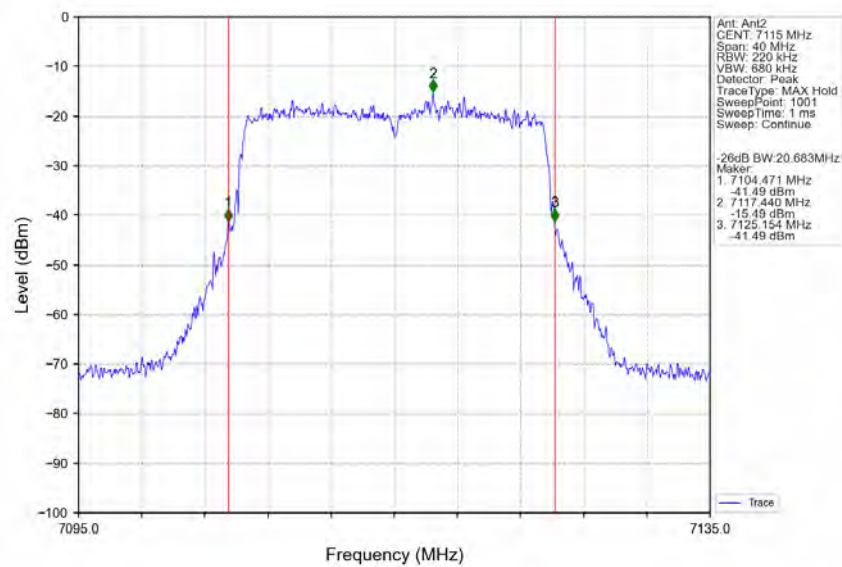
802.11ax(HEW20)_HCH_7115MHz_RU242_Left_Ant2_NTNV
