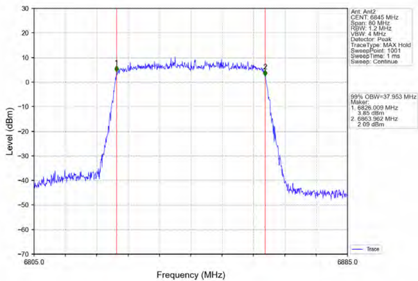
802.11ax(HEW40)_HCH_6845MHz_RU484_Left_Ant2_NTNV
