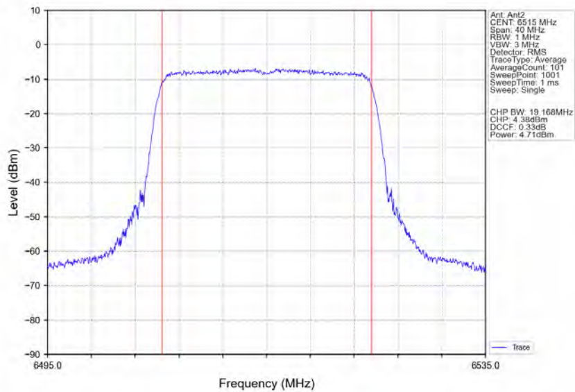
802.11ax(HEW20)_HCH_6515MHz_RU242_Left_Ant2_NTNV
