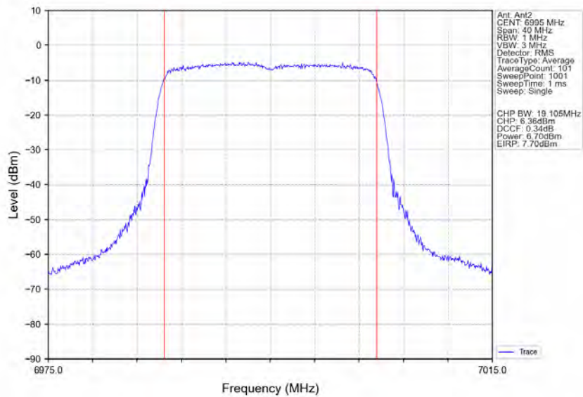
802.11ax(HEW20)_MCH_6995MHz_RU242_Left_Ant2_NTNV
