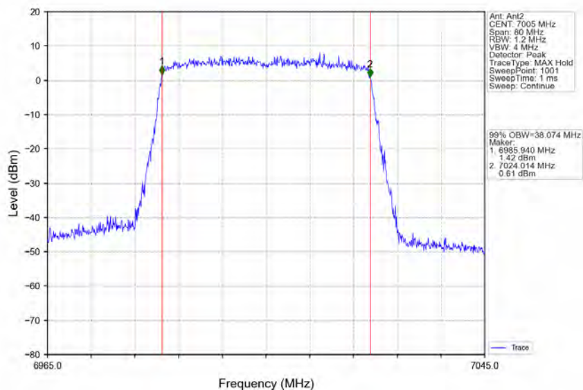
802.11ax(HEW40)_MCH_7005MHz_RU484_Left_Ant2_NTNV
