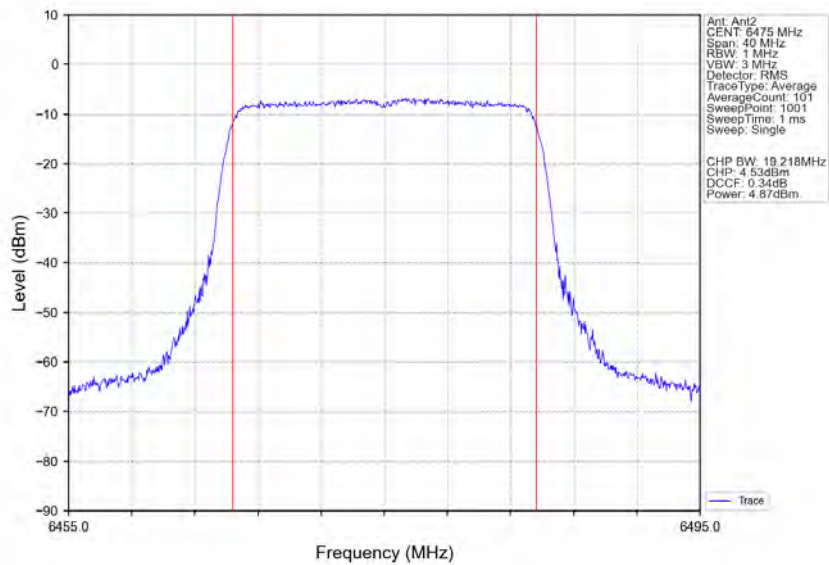
802.11ax(HEW20)_MCH_6475MHz_RU242_Left_Ant2_NTNV
