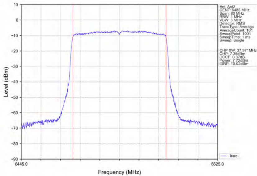
802.11ax(HEW40)_MCH_6485MHz_RU484_Left_Ant2_NTNV
