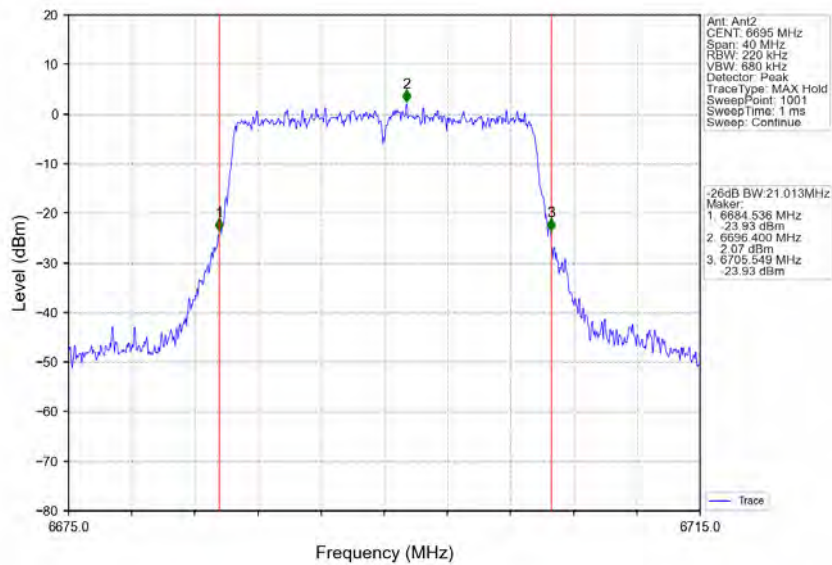
802.11ax(HEW20)_MCH_6695MHz_RU242_Left_Ant2_NTNV
