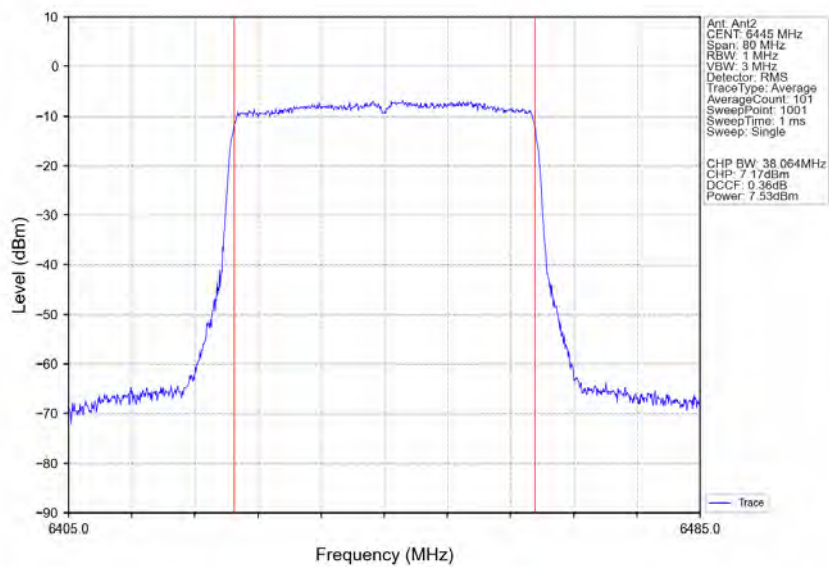
802.11ax(HEW40)_LCH_6445MHz_RU484_Left_Ant2_NTNV
