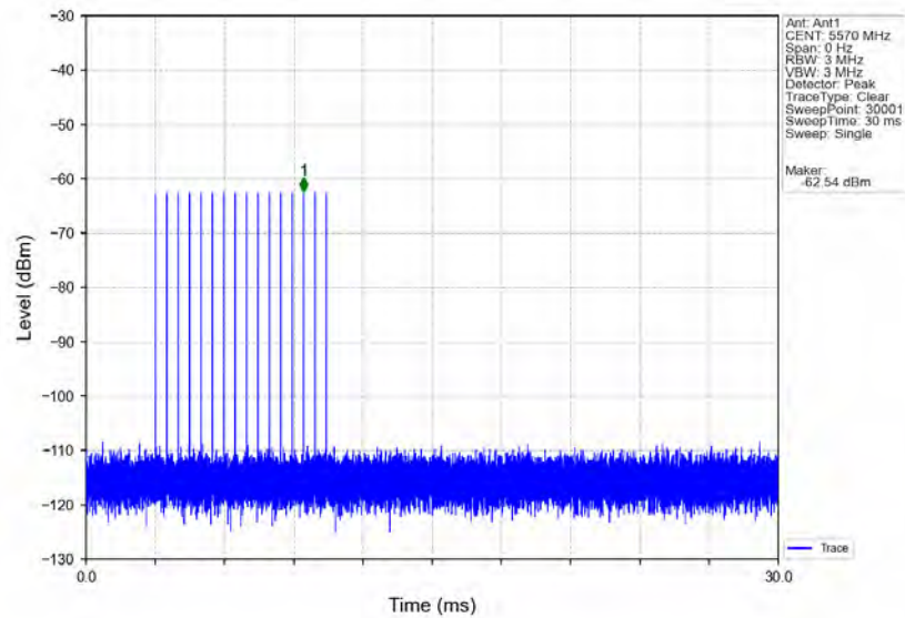
Signal Calibration_802.11ax(HEW160)_2C_5570MHz_RadarType5_Trial0
