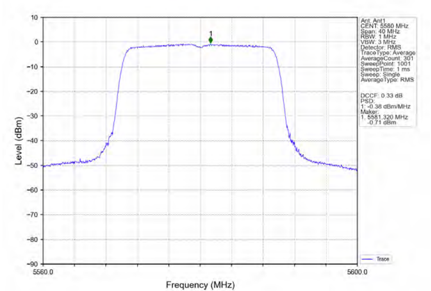
802.11ax(HEW20) MCH 5580MHz RU242 Left Ant1 NTN
