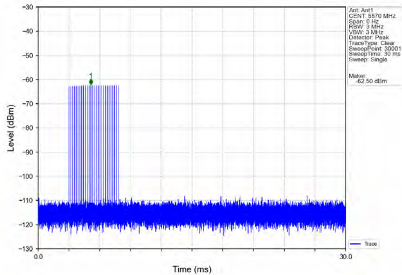
Signal Calibration_802.11ax(HEW160)_2C_5570MHz_RadarType3_Trial0
