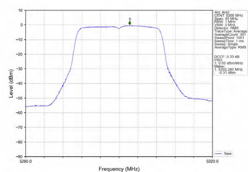
802.11ac(VHT20) MCH_5300MHz_Ant2_NTNV
