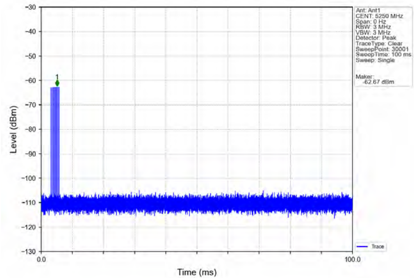
Signal Calibration 802.11ax(HEW160) 2A 5250MHz RadarType6 Trial0
