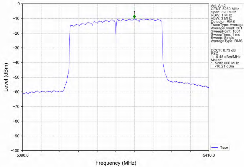
802.11ax(HEW160) MCH 5250MHz 2xRU996 Left MIMO NTN
