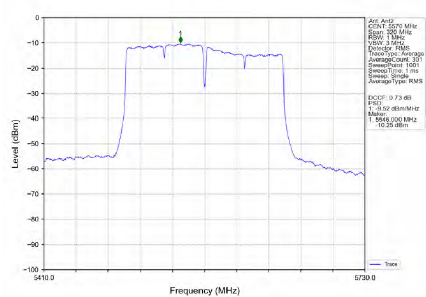
802.11ac(VHT160) MCH 5570MHz Ant2 NTN
