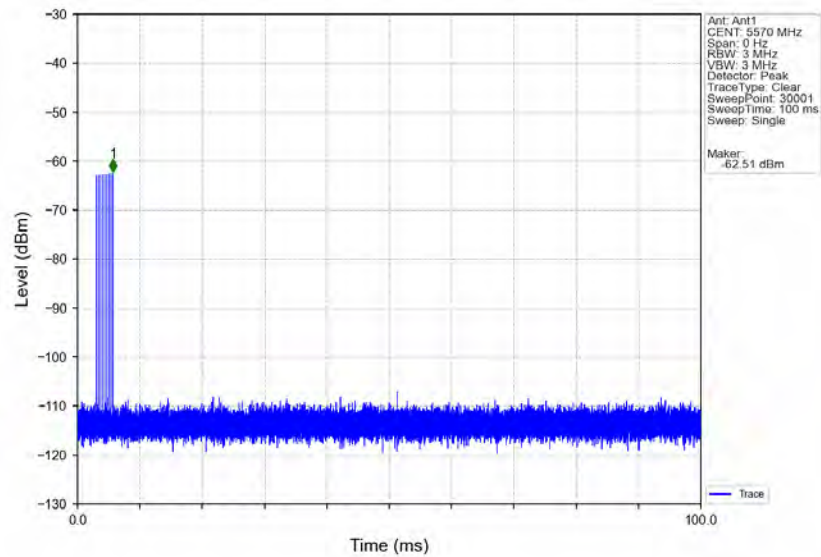
Signal Calibration 802.11ax(HEW160) 2C 5570MHz RadarType6 Trial0
