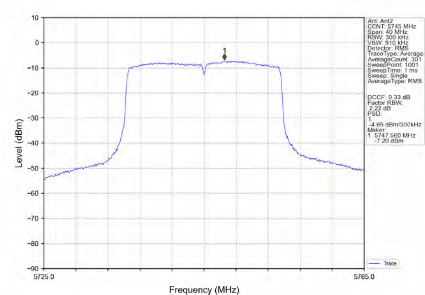
802.11ax(HEW20) LCH 5745MHz RU242 Left Ant2 NTN
