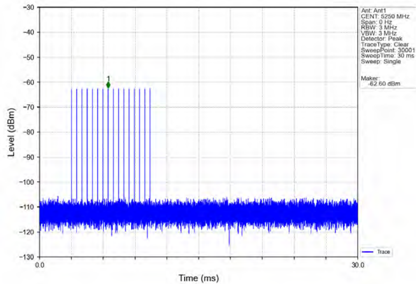
Signal Calibration_802.11ax(HEW160)_2A_5250MHz_RadarType5_Trial0
