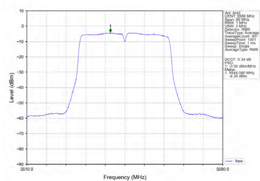
802.11ac(VHT40) MCH_5550MHz_Ant2_NTNV
