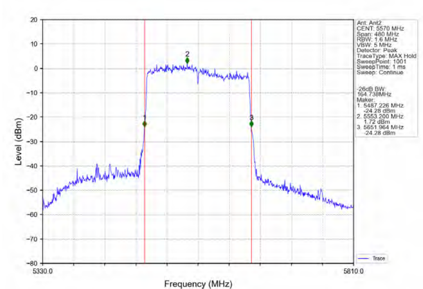
802.11ax(HEW160) MCH 5570MHz 2xRU996 Left Ant2 NTN
